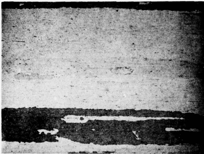
FIGURE 9: Microstructure of Alloy 44. Bar V144B extruded 2150°F (1175°C)/18:1/4.0 ips (10.2 cm/s) zone annealed 2360°F (1295°C)/2.8 ips (7.1 cm/s). Etchant: 45:45:10, HCl:H 2 O:H 2 O 2
