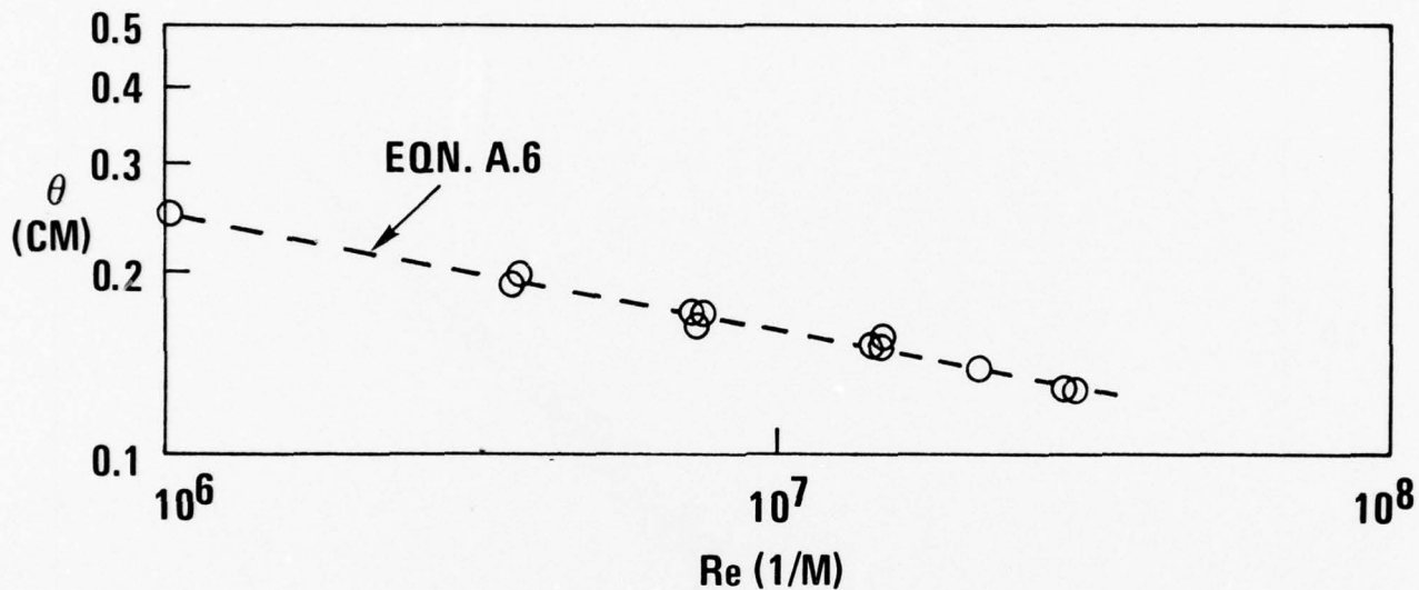
FIGURE A-3a BOUNDARY LAYER MOMENTUM THICKNESS INTERPOLATION, K = 0
