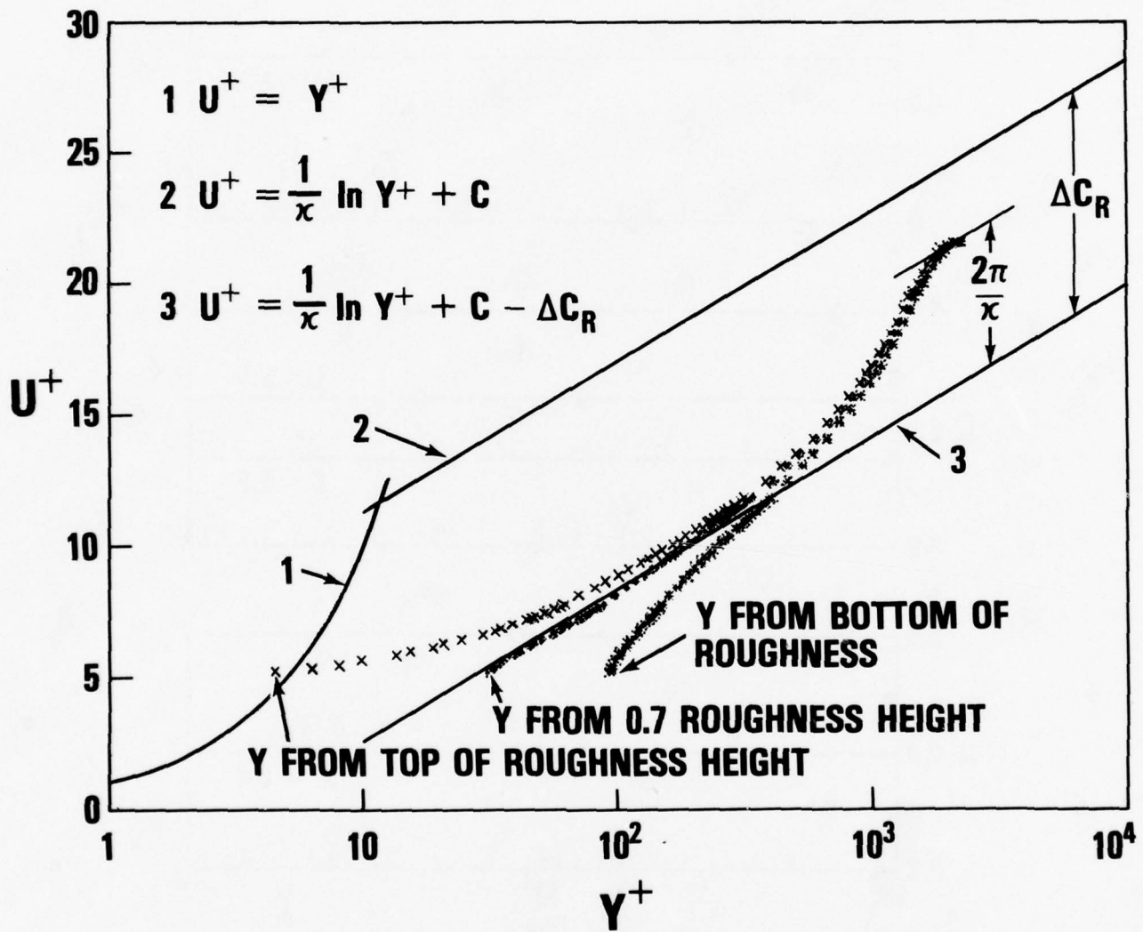
FIGURE 30 TYPICAL LAW-OF-THE-WALL PLOT WITH ROUGHNESS
