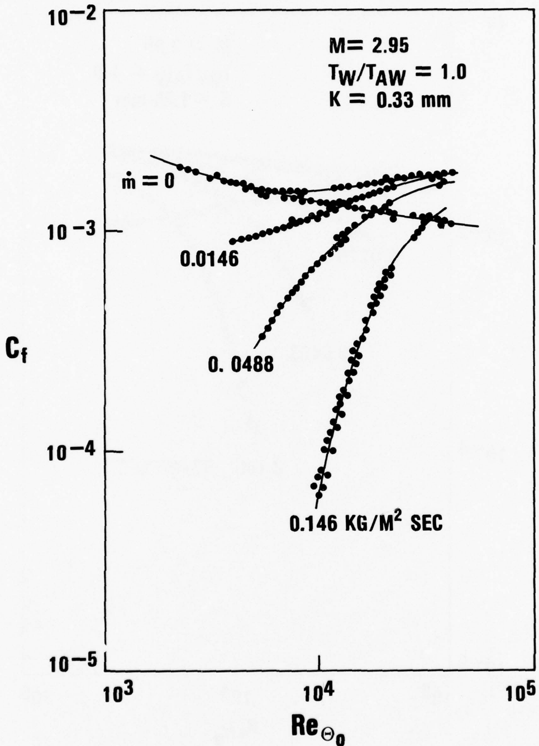
FIGURE 15 SKIN FRICTION DATA WITH BLOWING, K = 0.33 \text{ mm}
