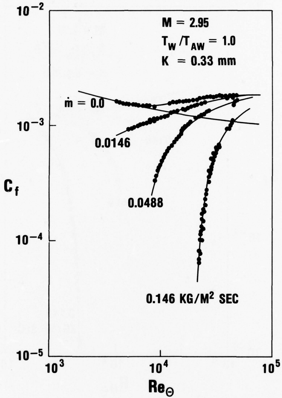
FIGURE 18 SKIN FRICTION DATA WITH BLOWING, K = 0.33 \text{ mm}
