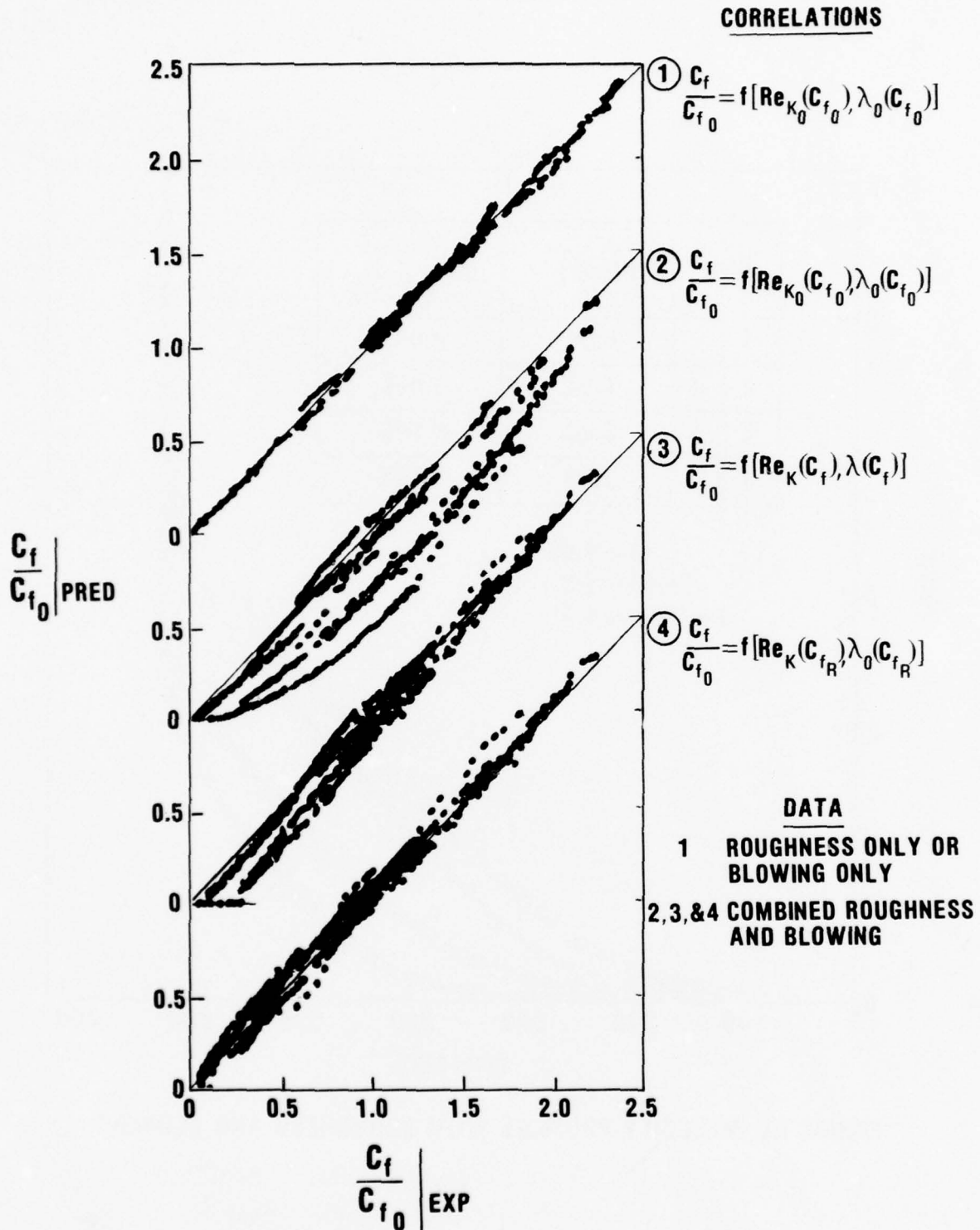
FIGURE 25 A COMPARISON OF PREDICTED AND MEASURED SKIN FRICTION USING INDEPENDENT CORRELATION SCHEMES
