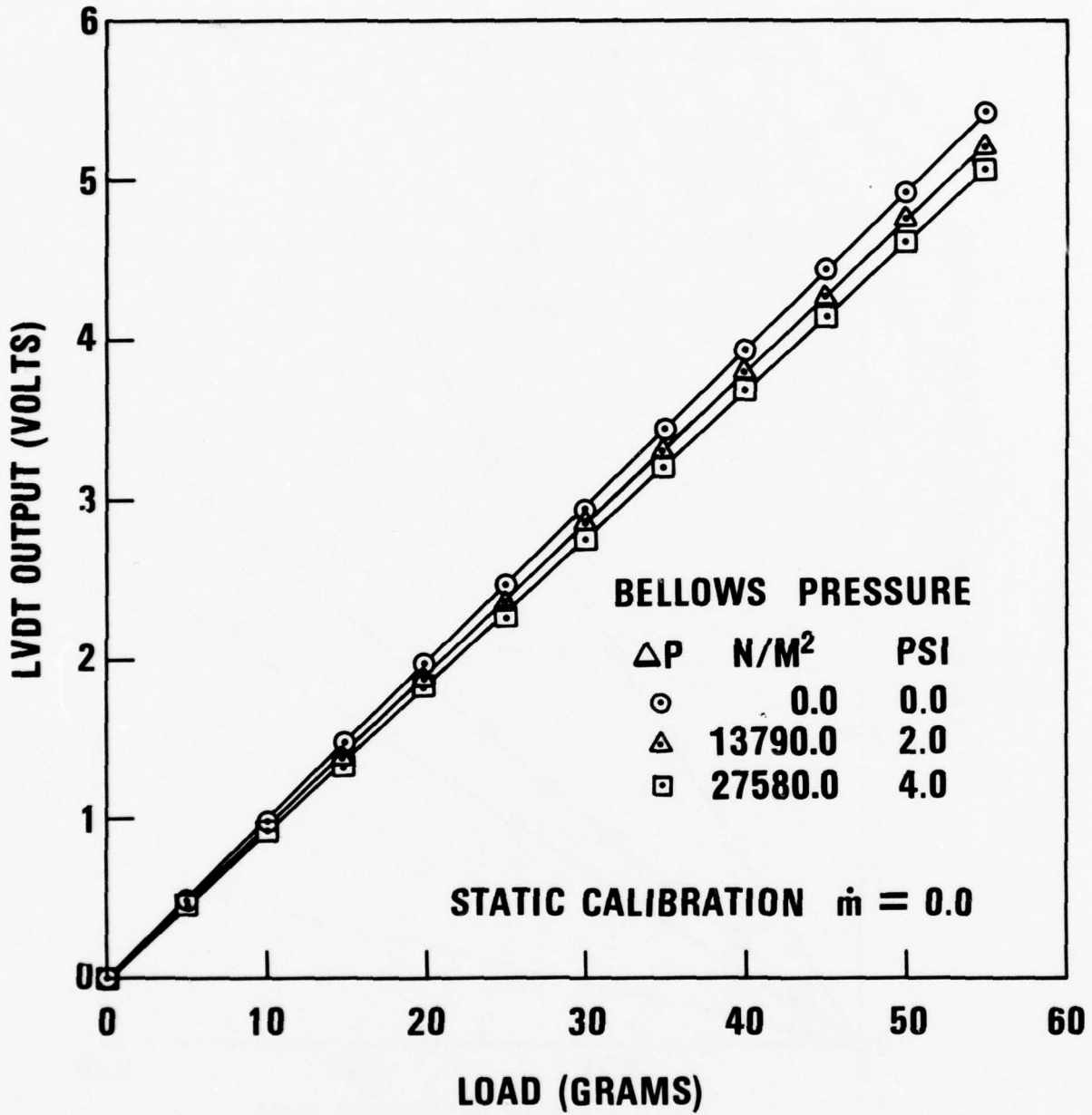
FIGURE 10a LOAD CALIBRATION SHIFT WITH BELLOWS PRESSURIZATION
