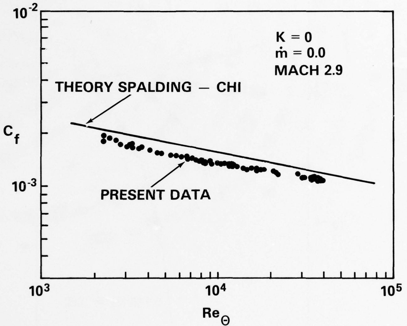
FIGURE 13 SMOOTH-WALL, NON-BLOWING SKIN FRICTION DATA
