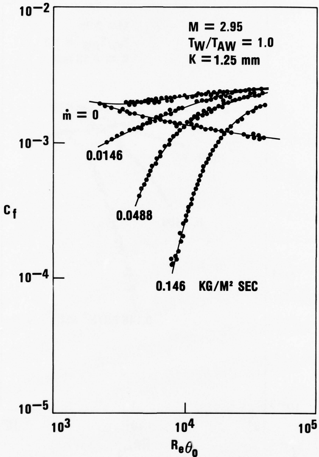
FIGURE 16 SKIN FRICTION DATA WITH BLOWING, K = 1.25 \text{ mm}
