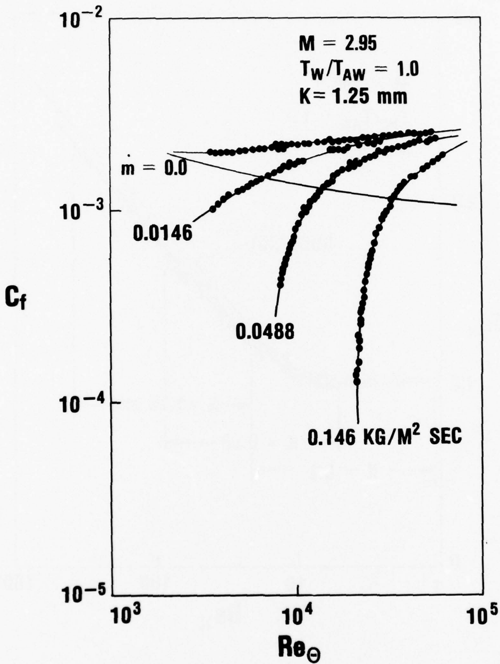
FIGURE 19 SKIN FRICTION DATA WITH BLOWING K = 1.25 \text{ mm}
