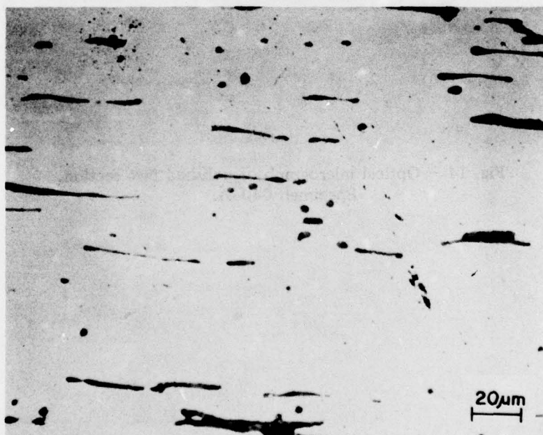
Fig. 16 — Optical micrograph of polished transverse section. Specimen 0404A.
