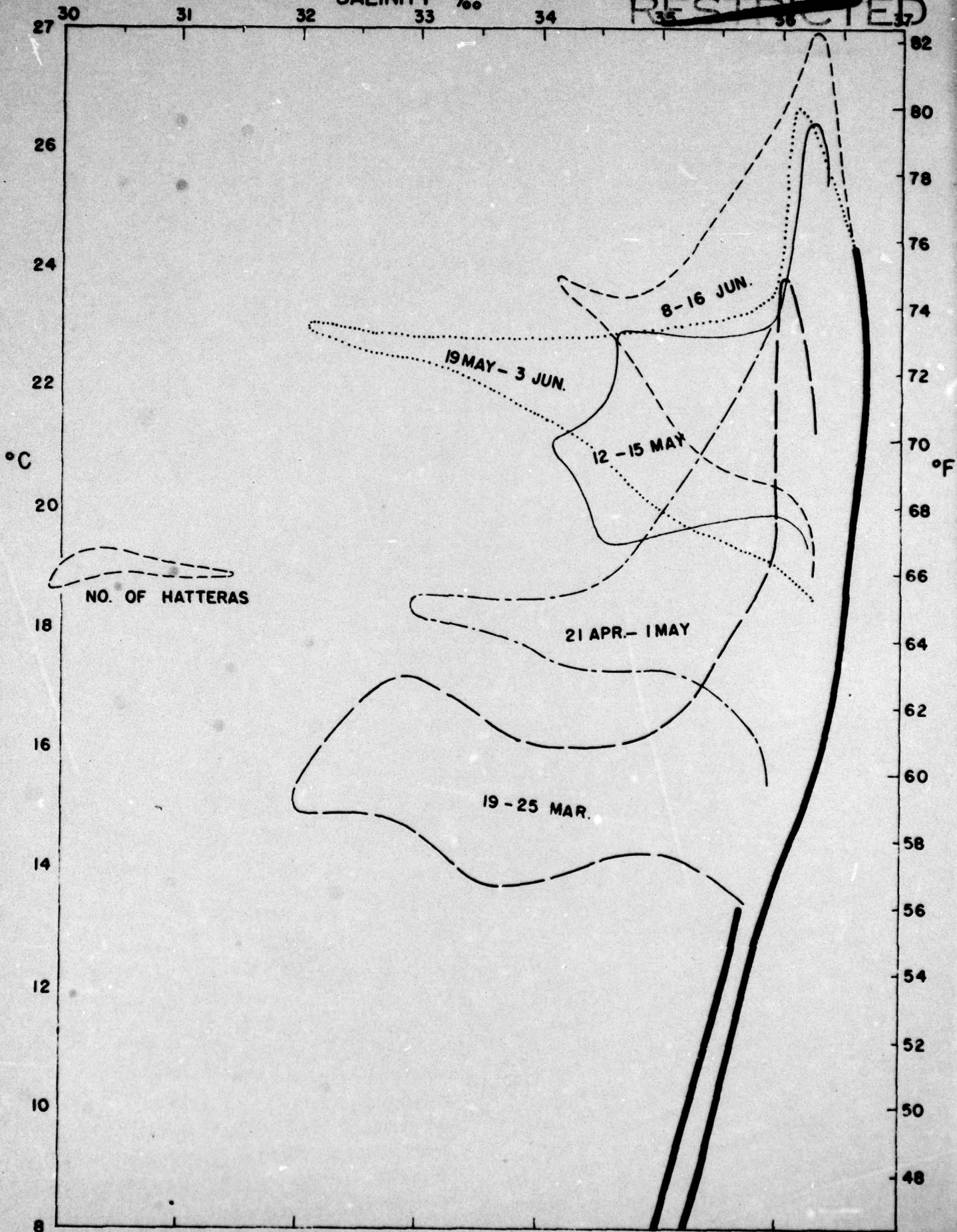
FIG. 1 T/S RELATIONS IN CAROLINA WATERS
