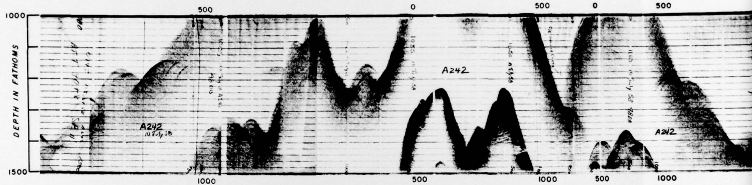
TOPOGRAPHY OF SEA FLOOR NORTHWEST OF CRETE LAT. 35° 35' N. LONG. 23° 30' E. APPROX.
