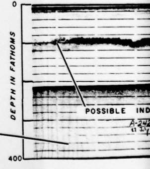
SCATTERING LAYER OBSERVED IN WESTERN MEDITERRANEAN SEA LAT. 40° 55' N. LONG 5° 10' E. APPROX.
