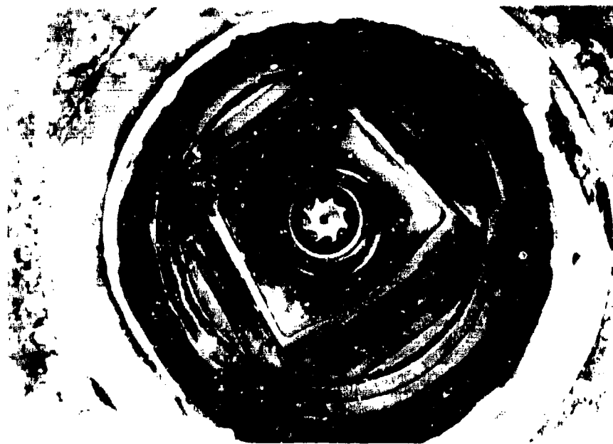
Figure B-12. Posttest Photograph of Swirl Cup After Carbon Deposition Test of Fuel 12.
