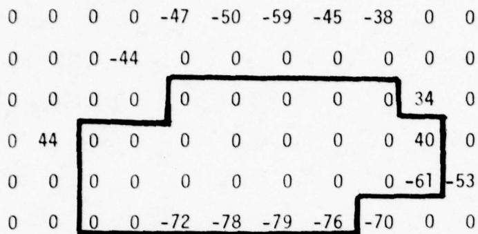
Figure 2.0-9b 4x4 Output
