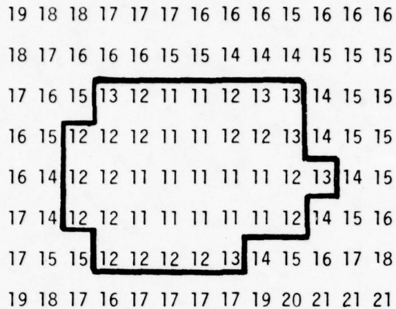
Figure 2.0-10a 5x5 Median Filter, Image 300, t \leq 13
