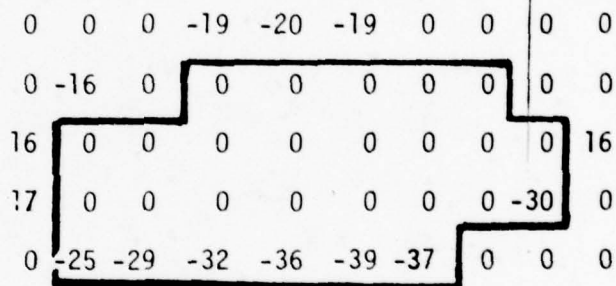
Figure 2.0-9c 2x2 Output
