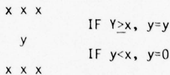
Figure 2.0-8 Non-Maximum Suppression
