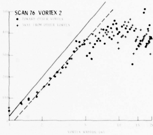
B-747 VORTEX, NORMAL LANDING CONFIGURATION
