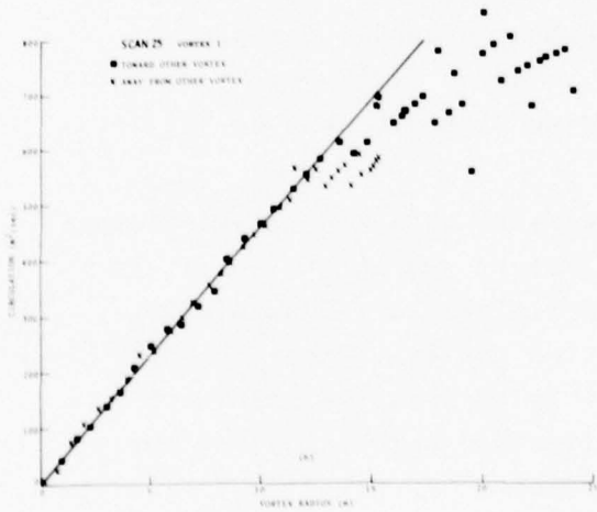
B-747 VORTEX, NORMAL LANDING CONFIGURATION SPOILERS DEPLOYED
