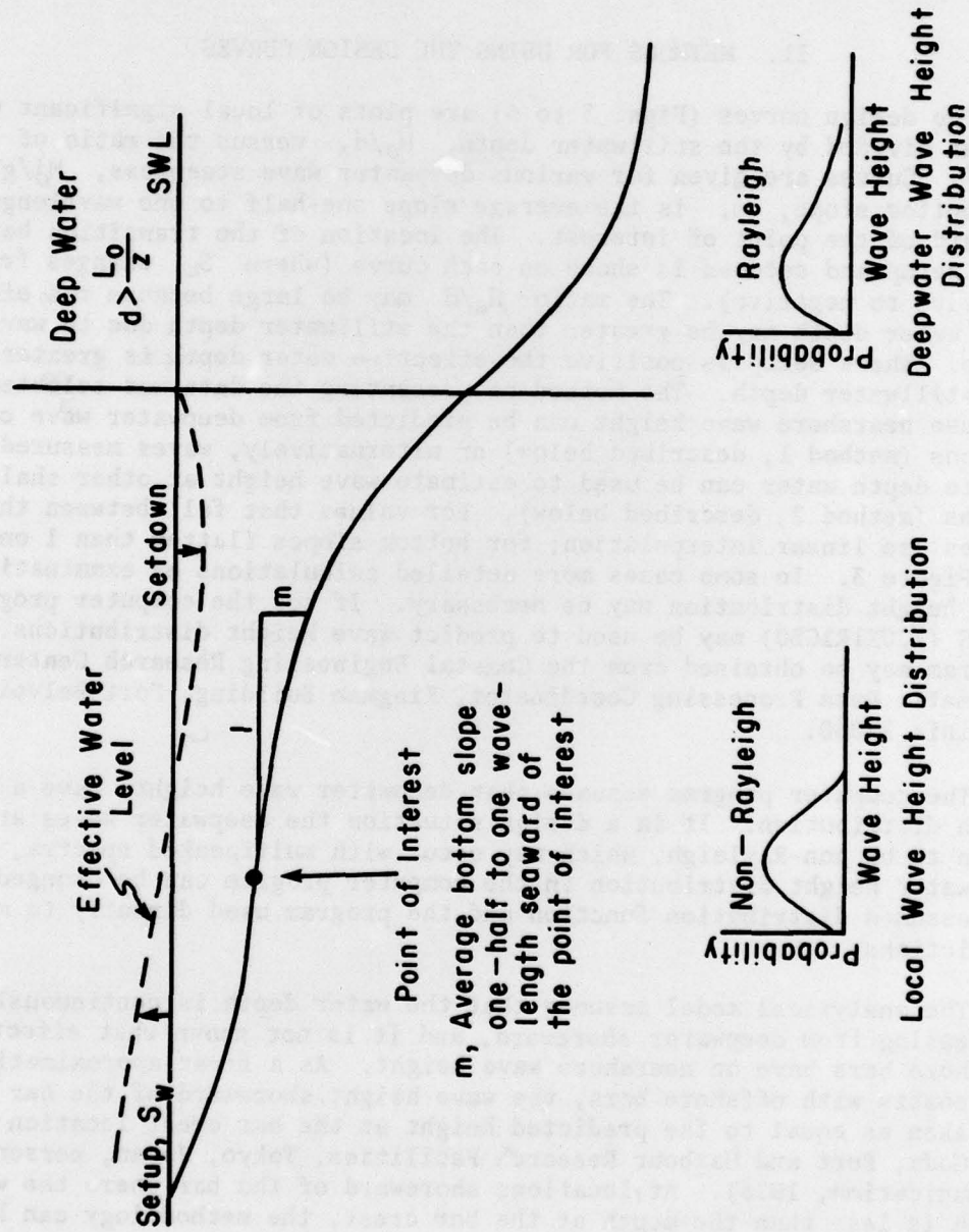
Figure 2. Conditions in the nearshore zone.
