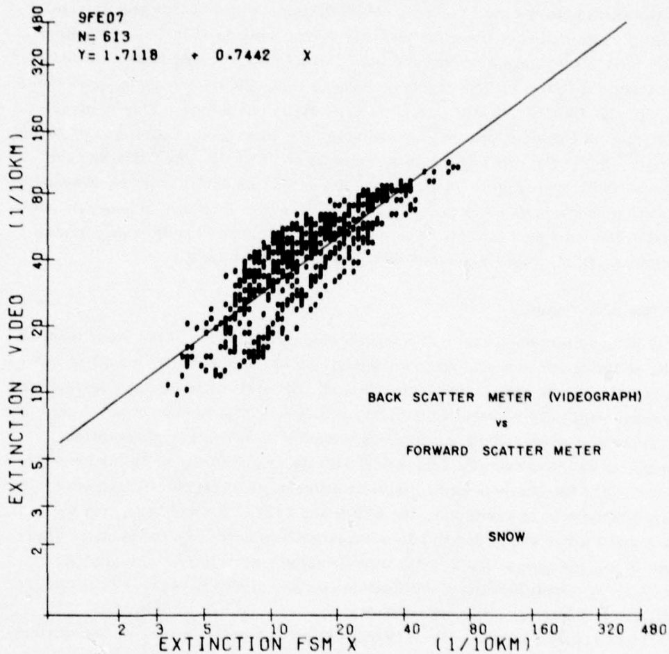
Figure 5. Comparison between Back Scatter Meter (Videograph) and Forward Scatter Meter Measurements (1-min Averages) of Atmospheric Extinction Coefficient during Snow
