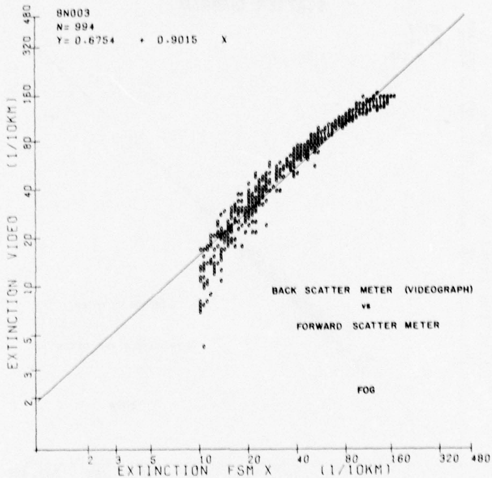
Figure 3. Comparison between Back Scatter Meter (Videograph) and Forward Scatter Meter Measurements (1-min Averages) of Atmospheric Extinction Coefficient during Fog
