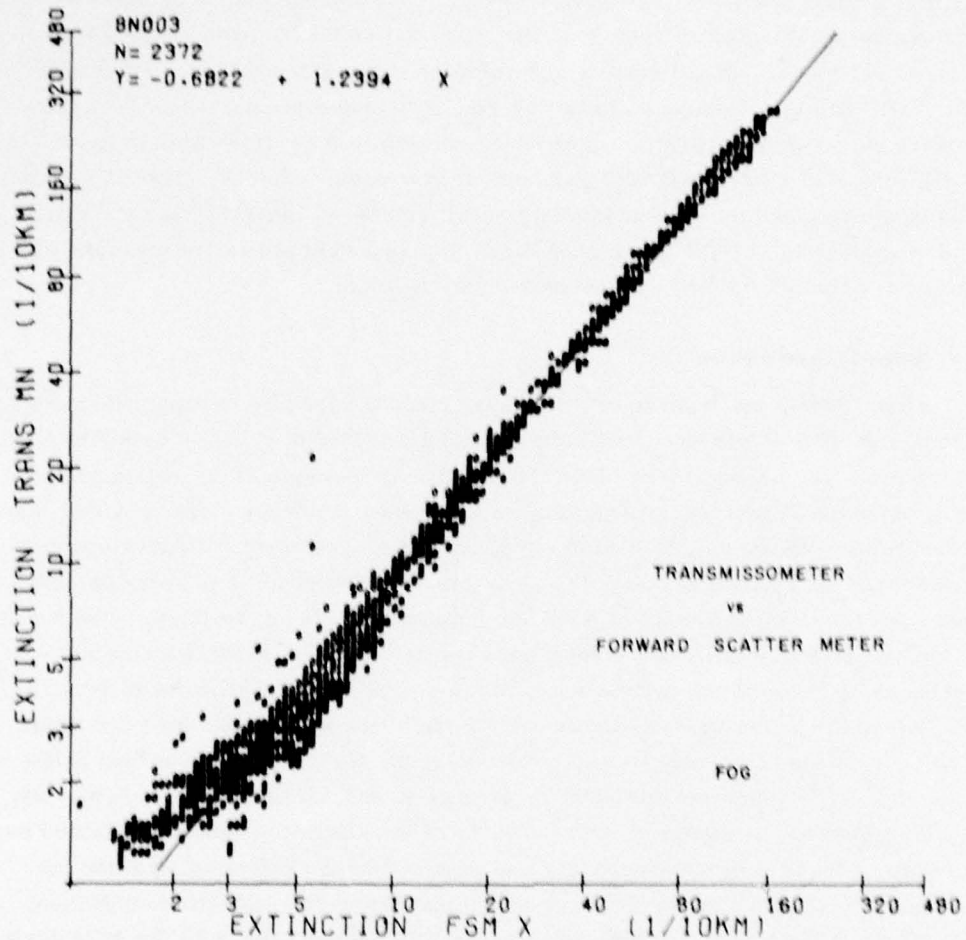
Figure 2. Comparison between Transmissometer and Forward Scatter Meter Measurements (1-min Averages) of Atmospheric Extinction Coefficient during Fog
