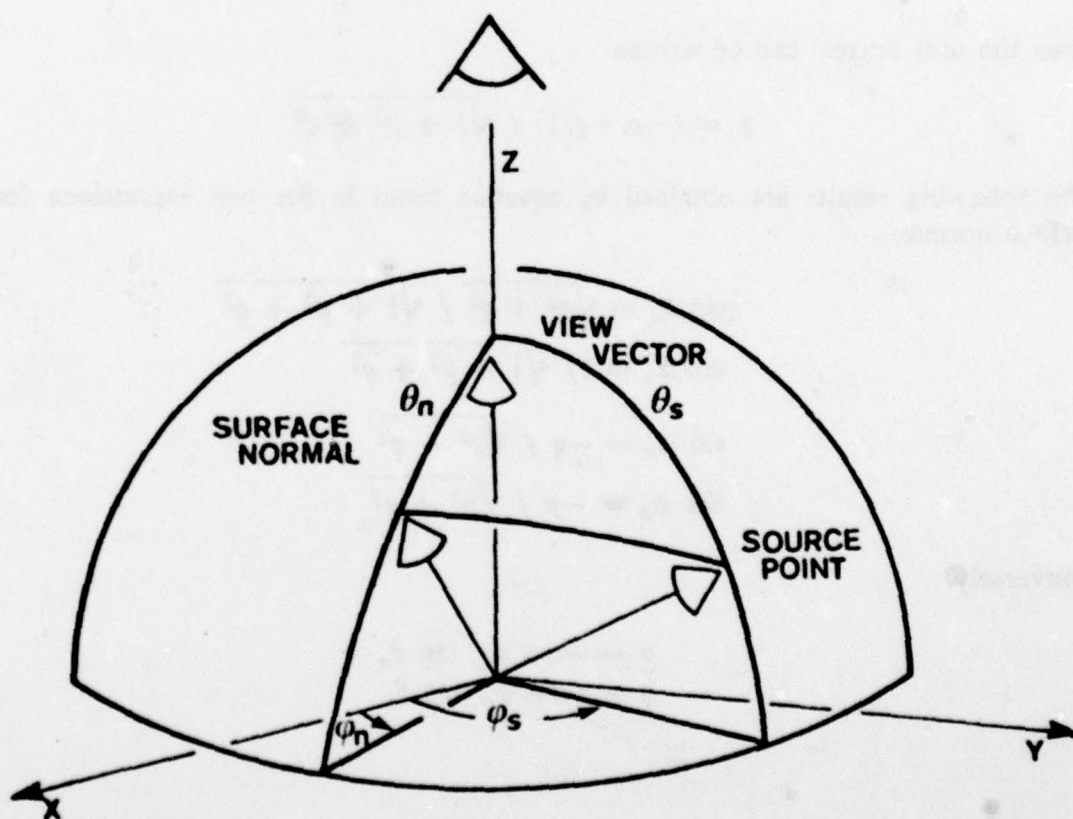
FIGURE 8: Surface normal and direction to portion of the source shown in viewer-oriented coordinate system.
