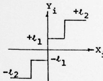
Fig. 4 4-level quantizer
