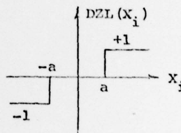
Fig. 2 A symmetric dead-zone limiter with dead-zone (-a, a)
