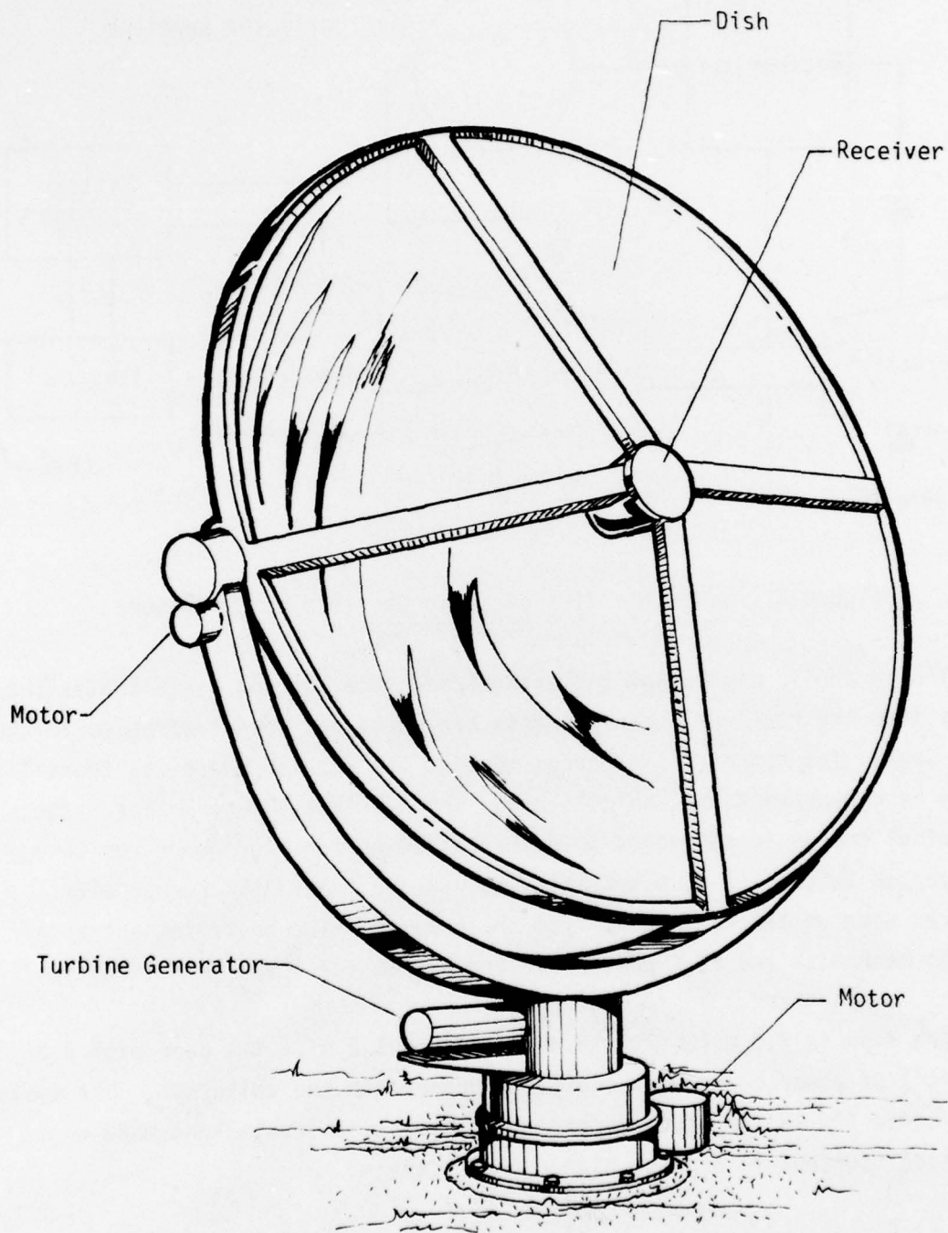
Figure 1. Concept of Individual Solar Gas-Turbine Power Module
