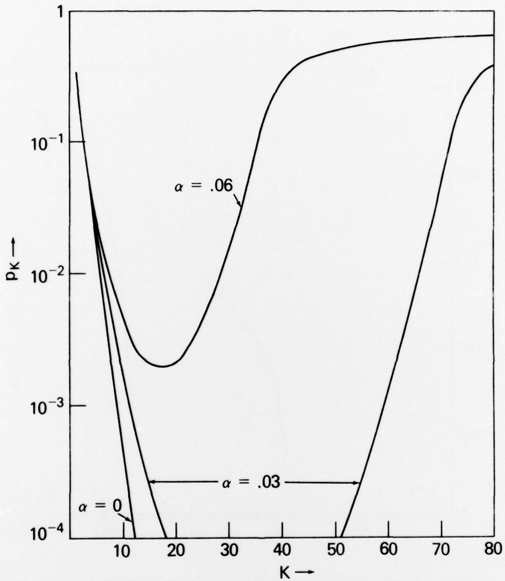
Fig. 4 — Probability that the system is full vs. system capacity K for three values of the linear overhead factor a . The load factor is \rho = .5 .
