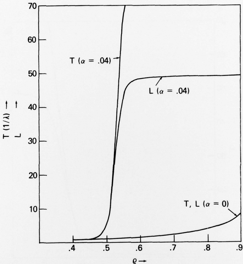
Fig. 2 — Expected number of customers L and expected system time T (in units of 1/\lambda ) vs. load factor \rho for linear overhead factors a = .04 and a = 0 with system capacity K = 50 . The a = 0 curves show performance for the overhead-free M/M/1/K case.
