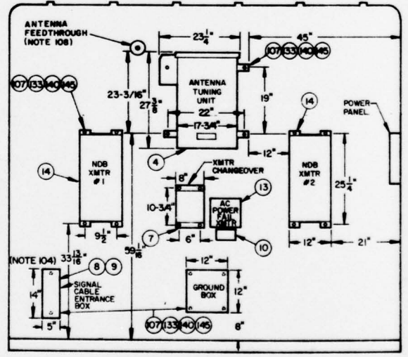
FIGURE 4 NDB EQUIPMENT MOUNTING DETAILS
