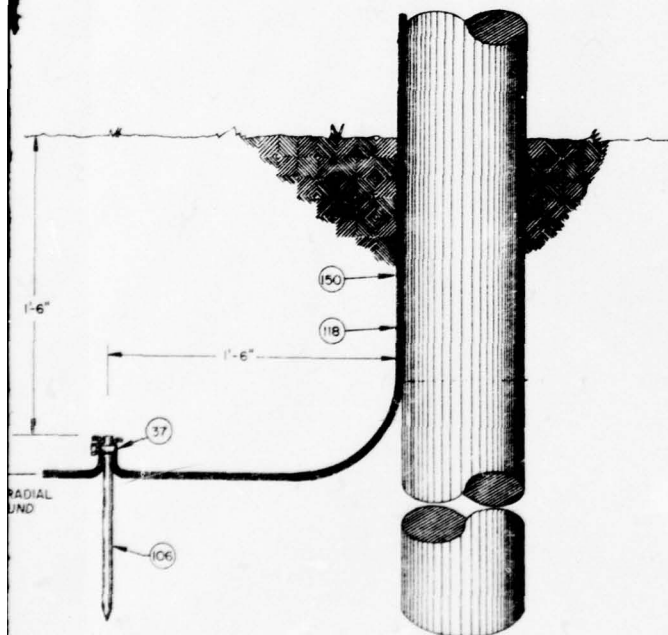
VIEW D-D GROUND ROD
