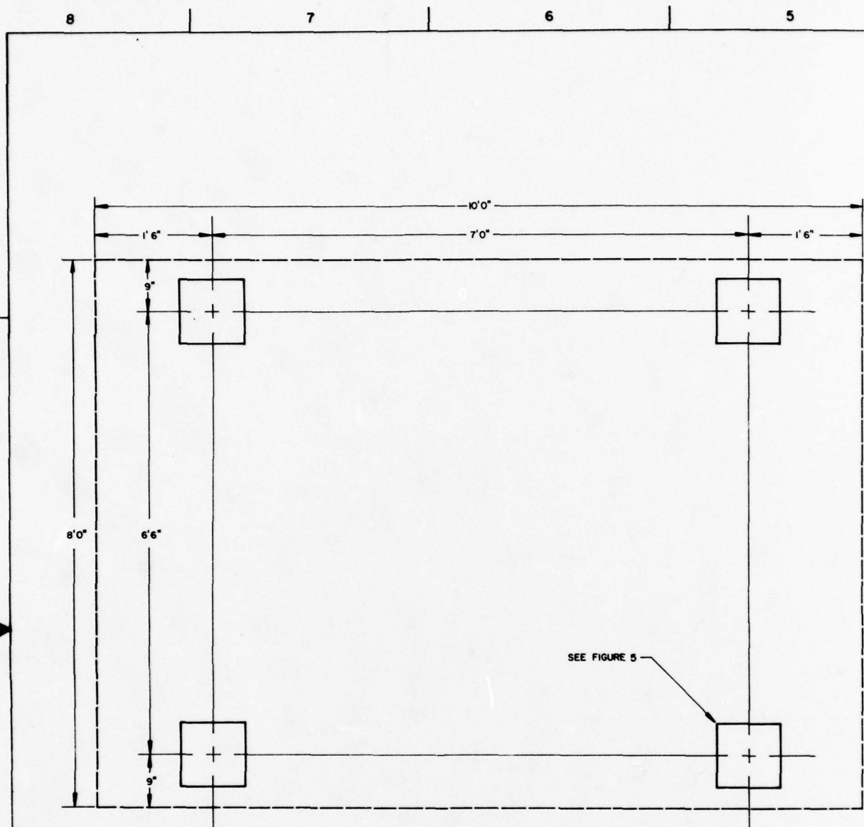
FIGURE 4 SHELTER FOUNDATION DETAILS
