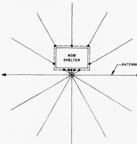
DETAIL A ALTERNATE ANTENNA & GROUND SYSTEM (NOTE 102)
