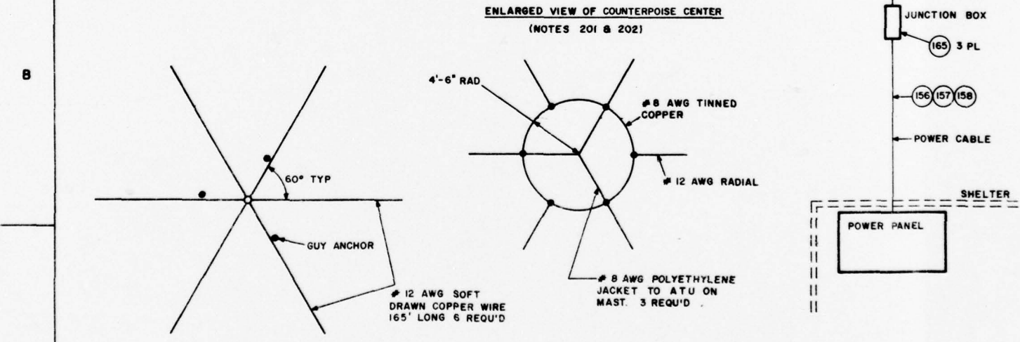
FIGURE 3 COUNTERPOISE INSTALLATION DETAILS
