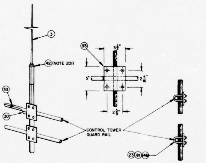
FIGURE 8 TYPICAL ANTENNA MOUNTING ON CONTROL TOWER GUARD RAIL
