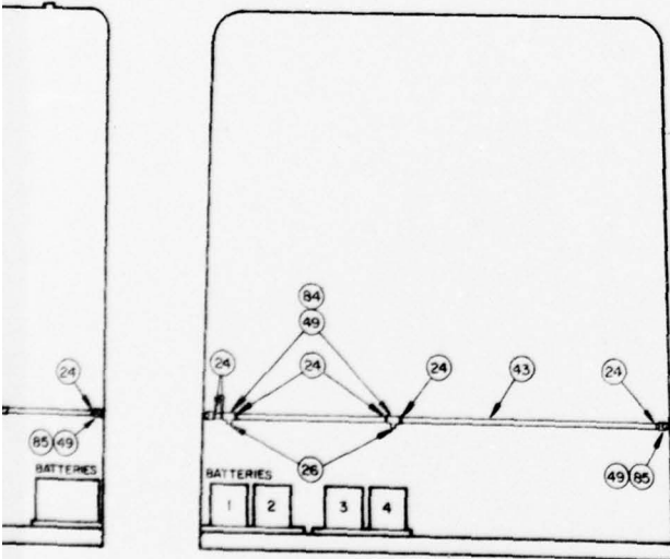
VIEW D-D BATTERY RACK CONDUIT INSTALLATION
