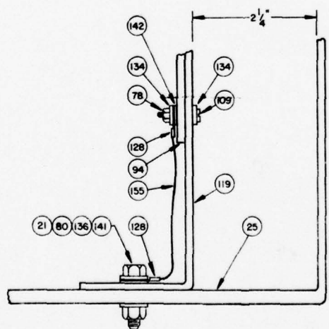
DETAIL L GROUND PLATE/SUPPORT BAR MOUNTING DETAILS
