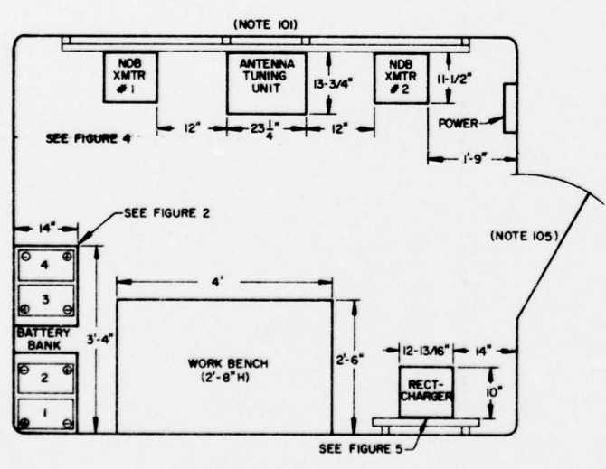
FIGURE 3 NDB SHELTER FLOOR PLAN LAYOUT
