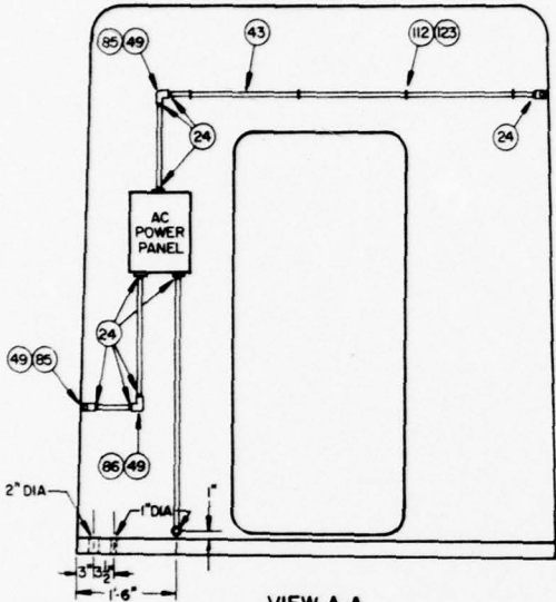
VIEW A-A AC POWER PANEL CONDUIT INSTALLATION (NOTE 103)
