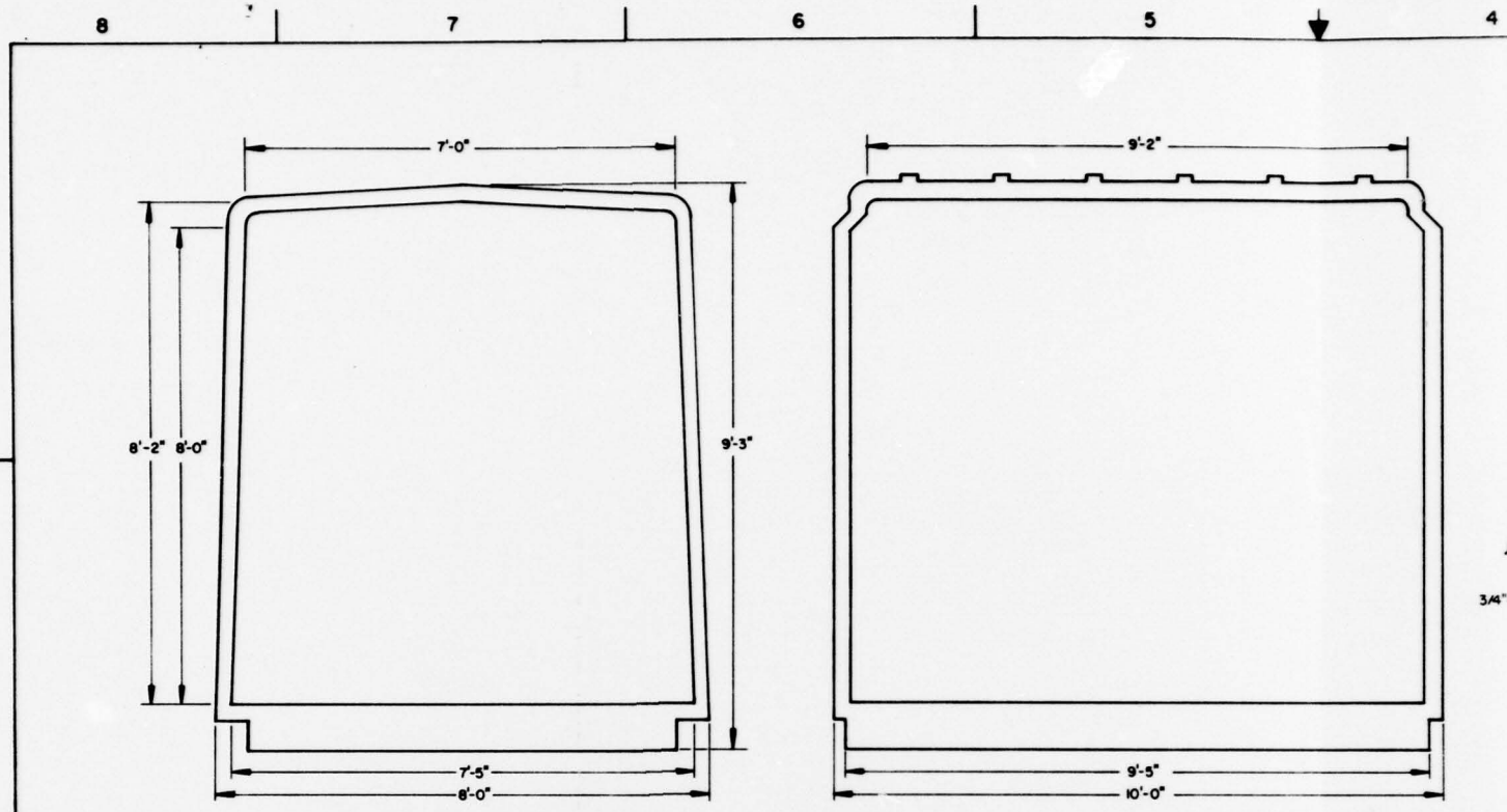
FIGURE 1 SHELTER LAYOUT (NOTES 106 & 107)
