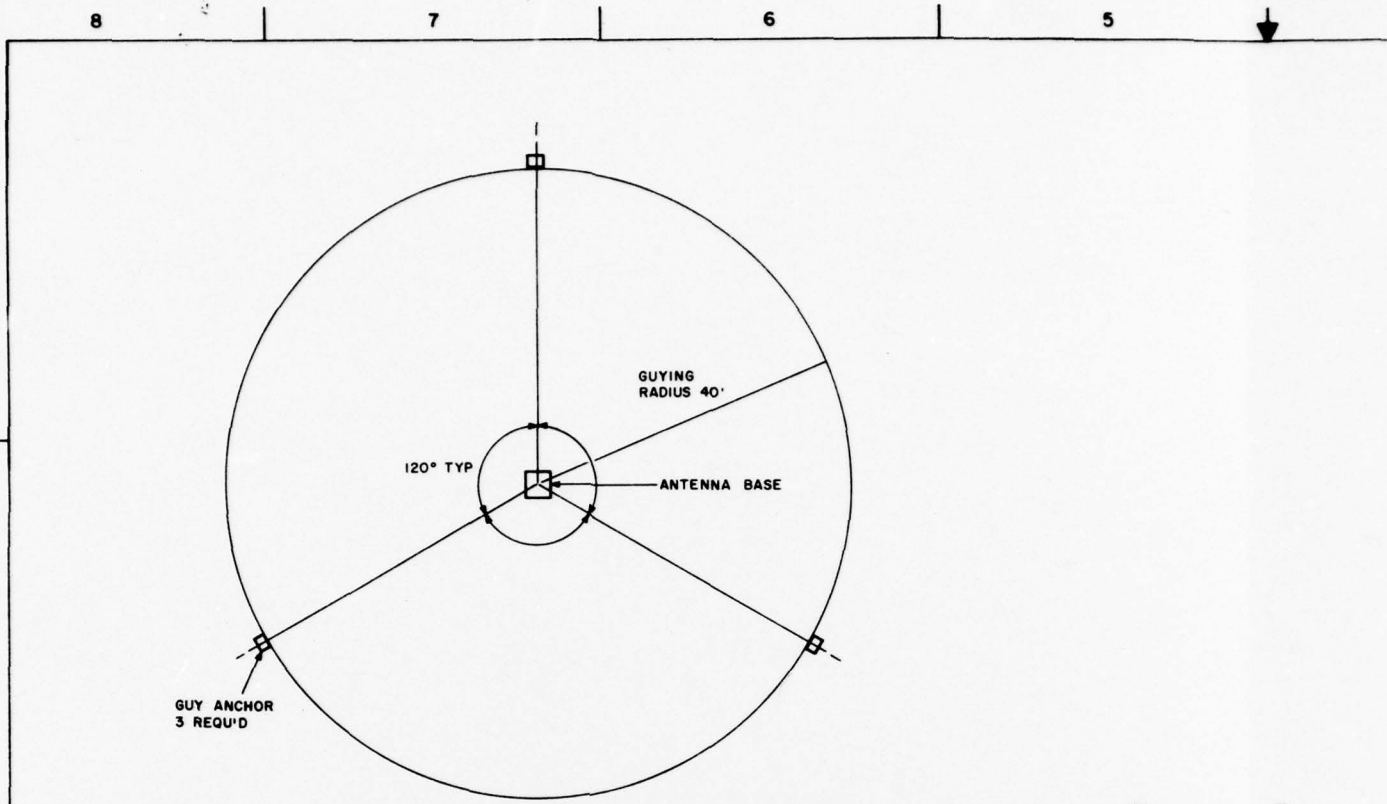
FIGURE 2 MAST GUYING LAYOUT
