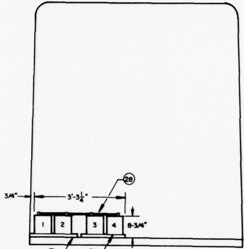
FIGURE 2 BATTERY BANK MOUNTING DETAILS
