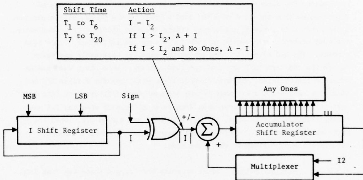
Figure 14. Digital Filter
