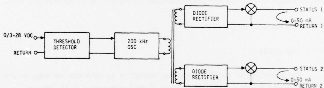
Figure 33. Status Hybrid Functional Flow Diagram
