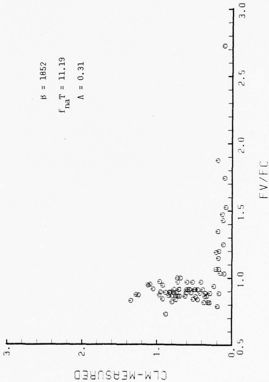
Fig. 18 C_{LM} versus \frac{f_v}{f_c} for a smooth cylinder
