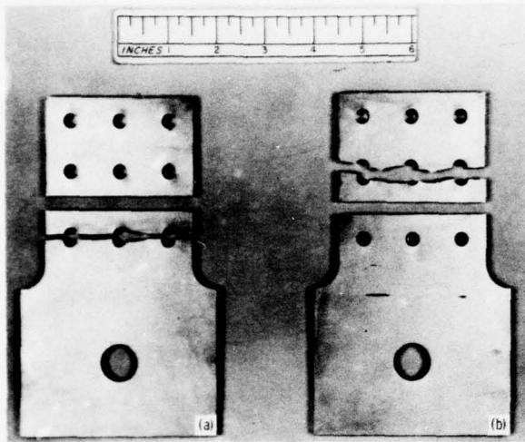
a. Three-hole joint
