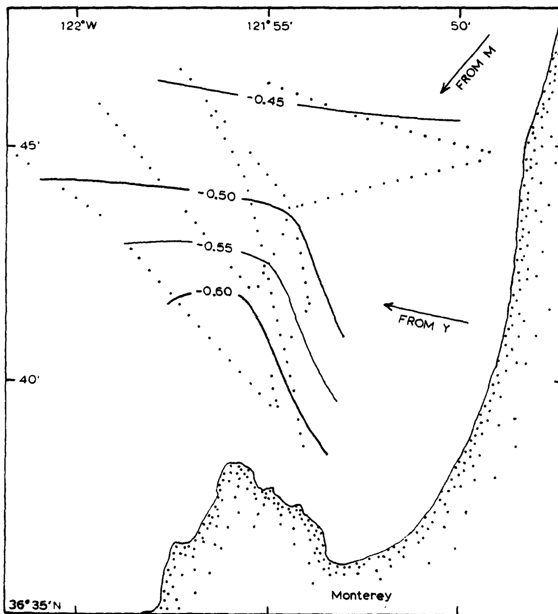
Figure 6. Overland Propagation Corrections, 9940-MHz Rate
