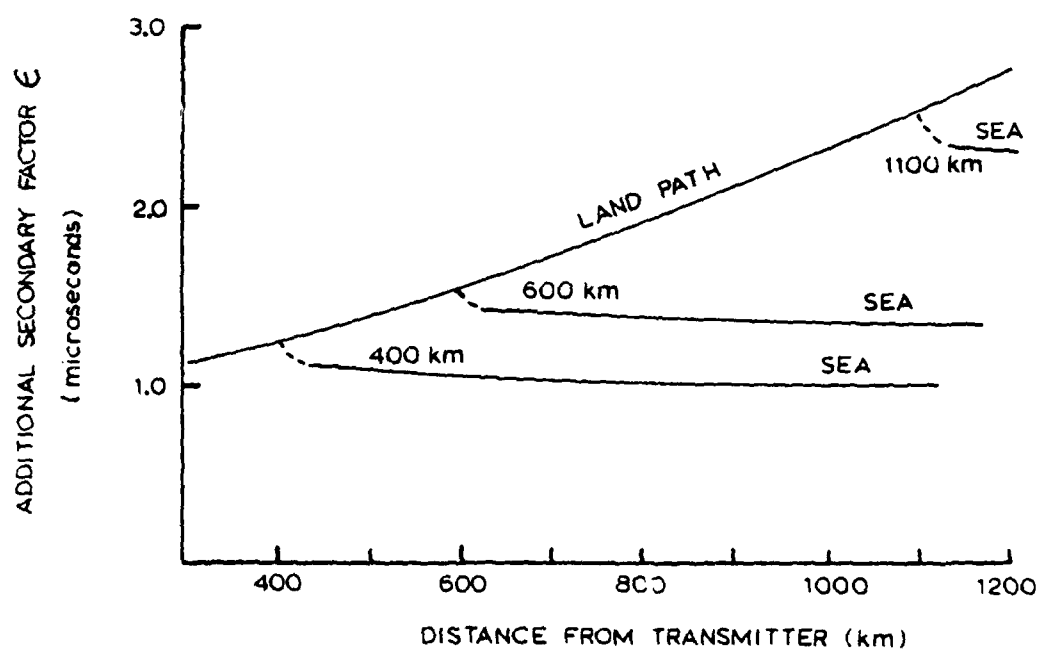
Figure 2. Variations of Additional Secondary Factor with Distance on Typical Land-Sea Paths
