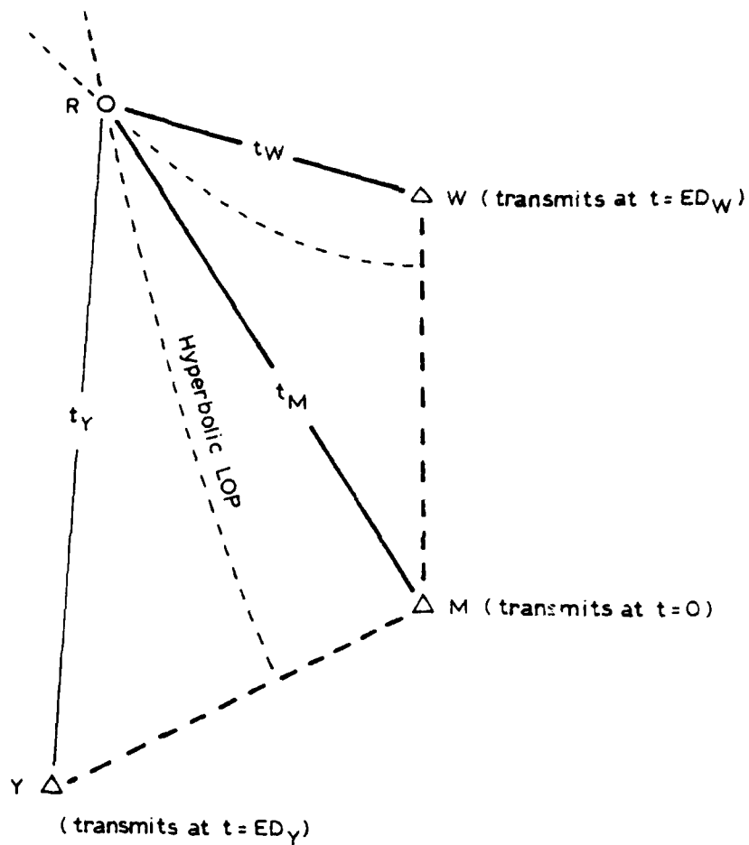
Figure 1. Components of Time Difference Measurement Loran transmitters located at W , M and Y and Receiver at R . Refer to text for explanation.
