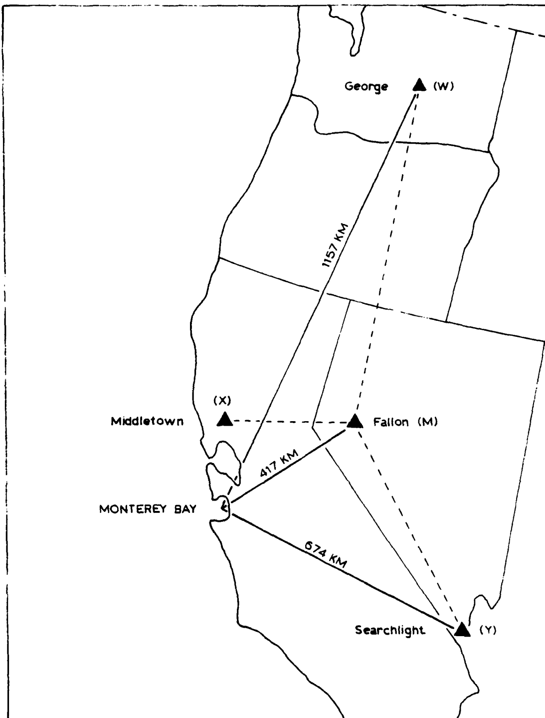
Figure 4. Location of West Coast Loran-C Stations
