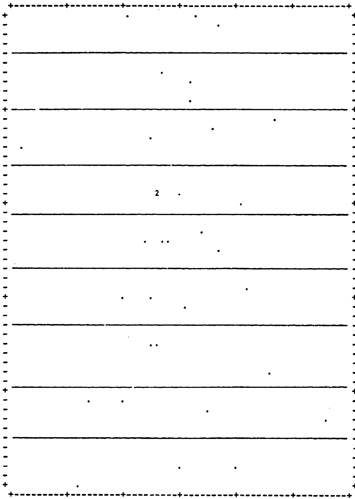
Figure 5. \hat{U} without intercept vs. natural log of quantity
