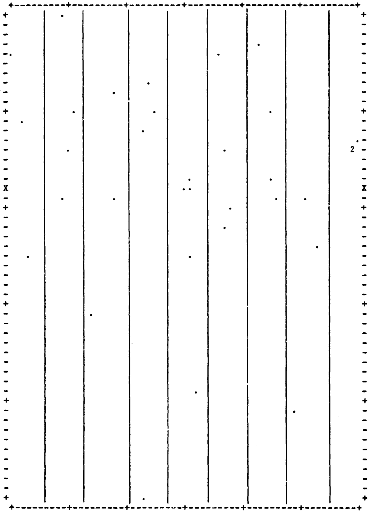
Figure 1. Marcotte's residuals (ord.) vs. ln(quantity) (abs.)
