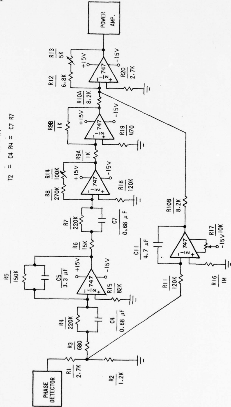
FIGURE 3 CIRCUIT DIAGRAM OF THE LAG-LEAD NETWORK, INTEGRATOR AND CARRIER FILTER
