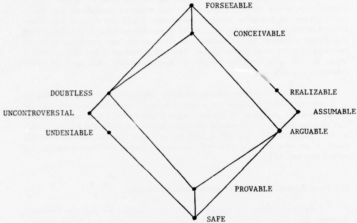
Figure 3. Diagram of the classifications of formulas. Each line connects a set of formulas with a superset.
