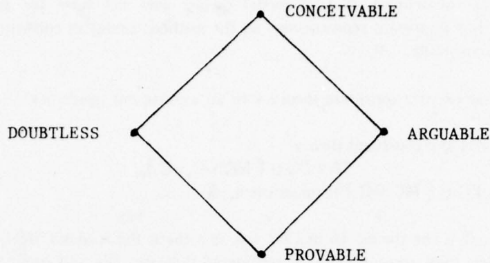
Figure 2. Diagram of four classifications of formulas. Each line connects a set of formulas with a superset. Incomparable sets are not connected in this way.
