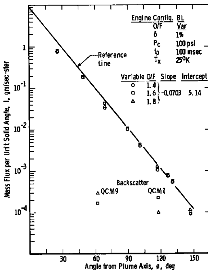
Figure 11. Effect of oxidizer-to-fuel ratio on mass flux.
