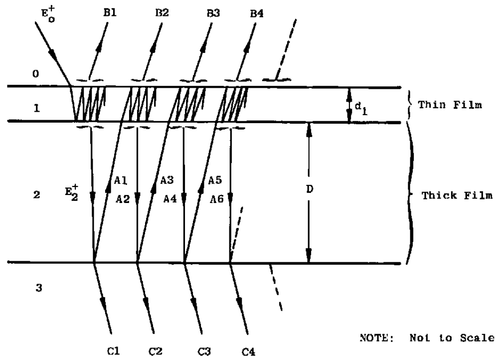
Geometry depicting analytical model for a thin film formed upon a thick film.
