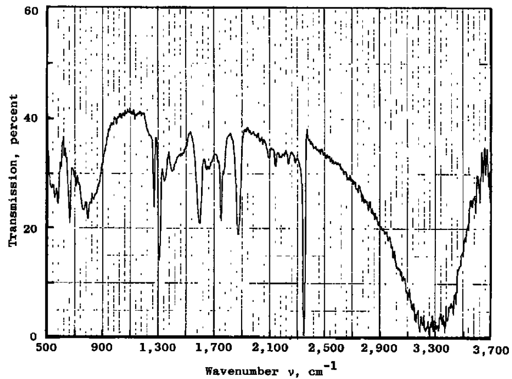
b. Germanium temperature = 96 to 103°K Figure 19. Continued.
