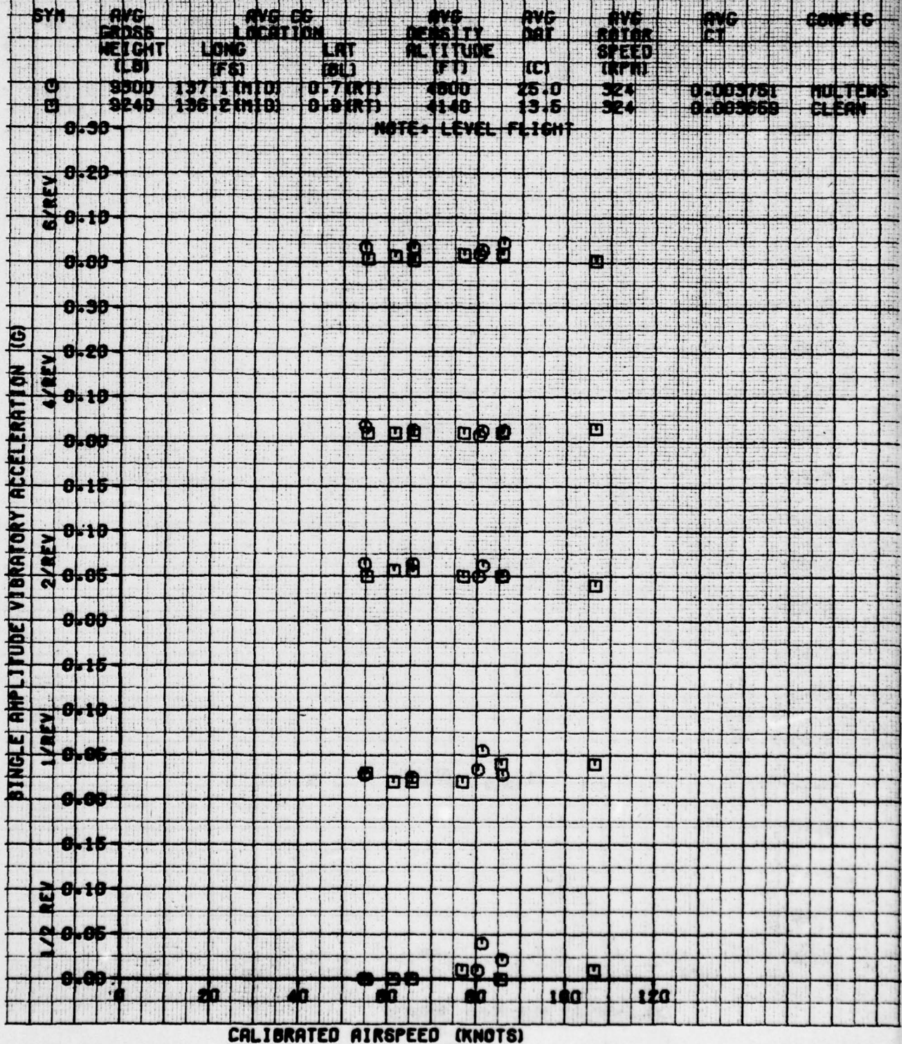
FIGURE 63 VIBRATION CHARACTERISTICS JUN-14 8/N 74-22358 PILOT FLOOR LATERAL
