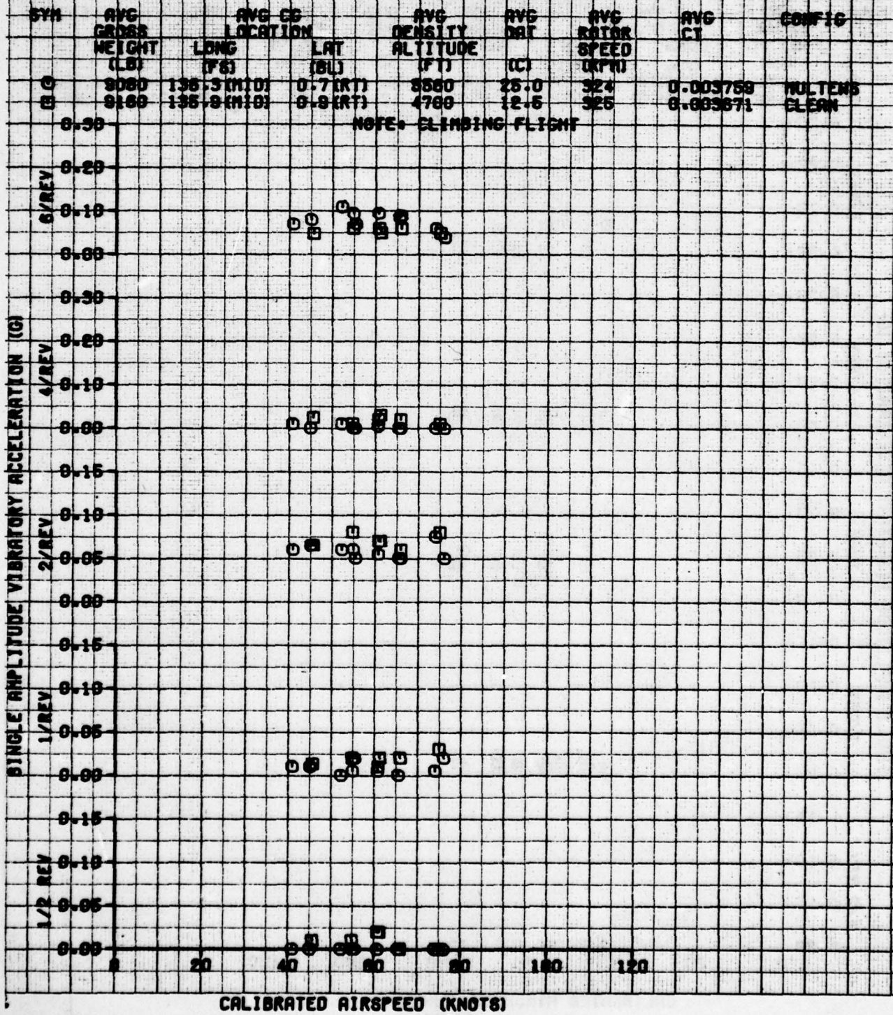
FIGURE 76 VIBRATION CHARACTERISTICS JHM-1H S/N 74-22338 C.G. FLOOR LONGITUDINAL
