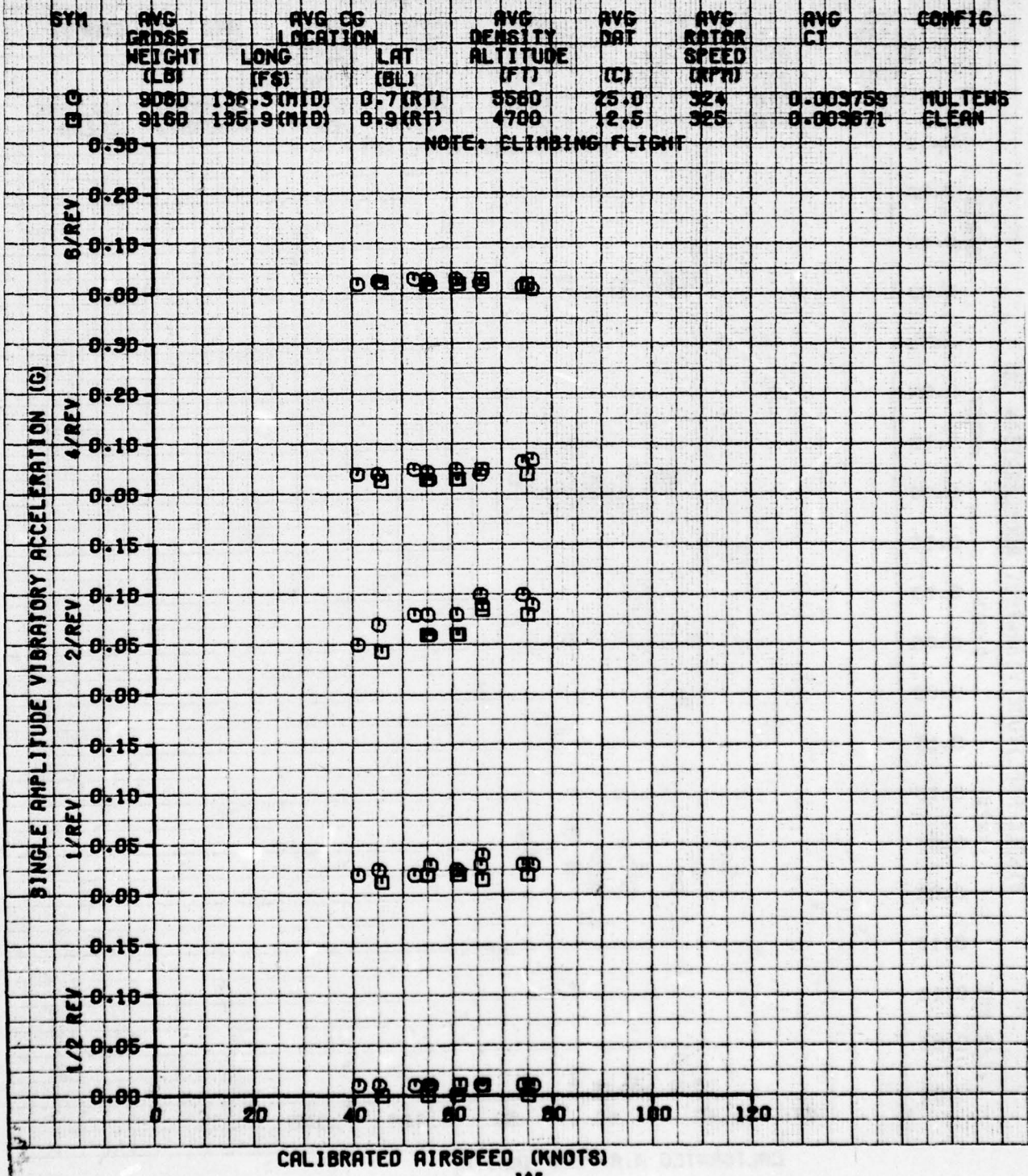
FIGURE 71 VIBRATION CHARACTERISTICS JUN-14 8/N 74-2238 PILOT FLOOR VERTICAL
