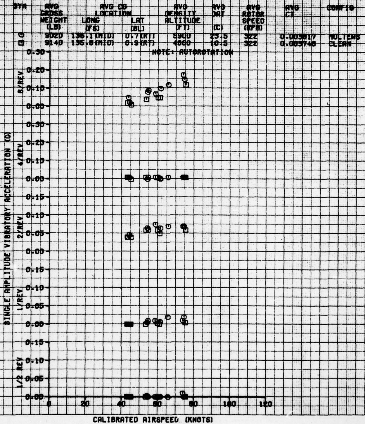
FIGURE 02 VIBRATION CHARACTERISTICS JUN-14 S/N 74-2238 PILOT FLOOR LONGITUDINAL
