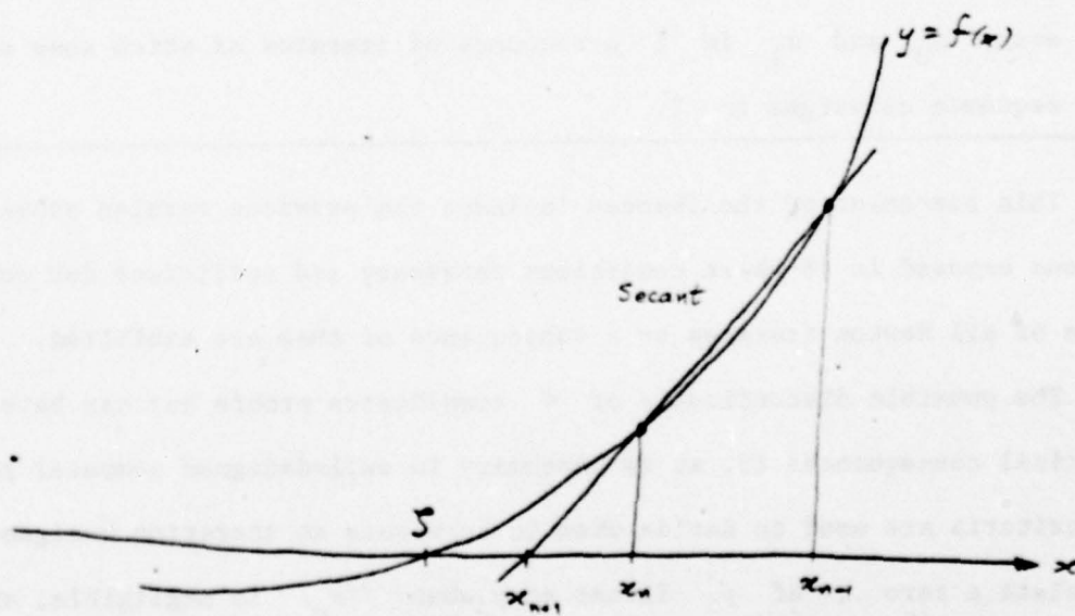
Fig. 7: Secant iteration
