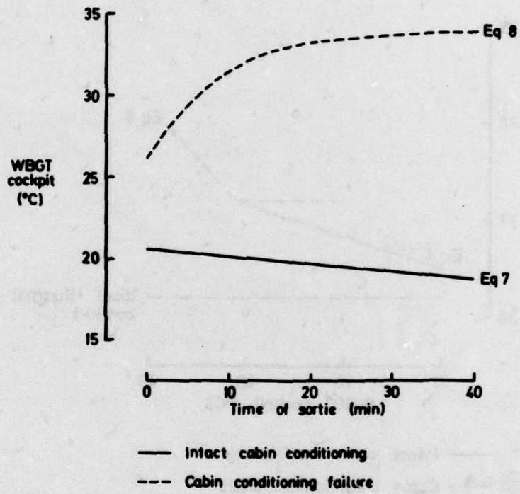
Figure 2 Relationship between cockpit WBGT and sortie time.
