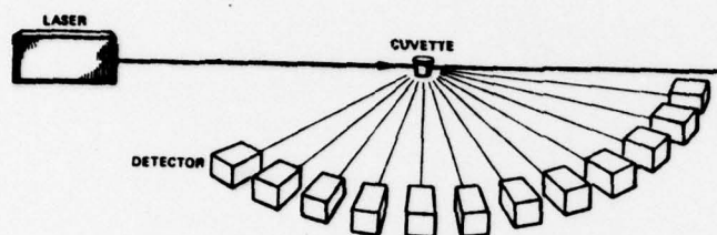
Fig. 1 - A schematic diagram of a differential light scattering measurement. The laser source illuminates a suspension of cells in a cuvette. Lying in a plane are the array detector elements, each of which measures the scattered intensity at a different angle, \theta , with respect to the incident laser beam.
