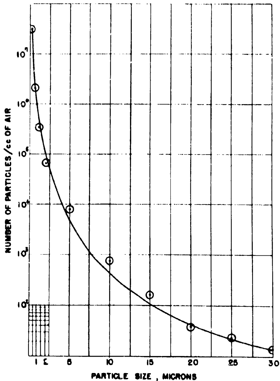
Fig. A.22 Pre-shock Dust Particle Size Distribution, Cascade Impactor, Station B-204-L
