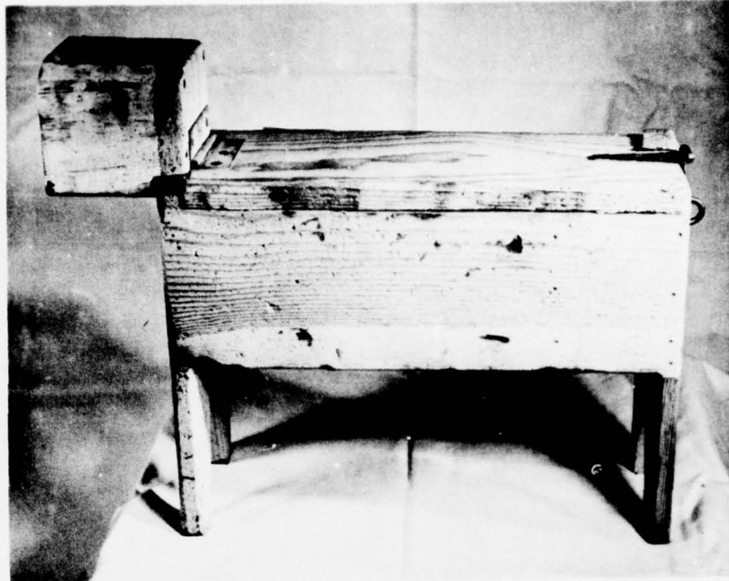
Fig. 1.4 Mock Dog, Side View
