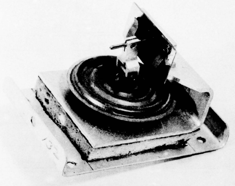
Fig. 1.7 Peak Pressure Recorder
