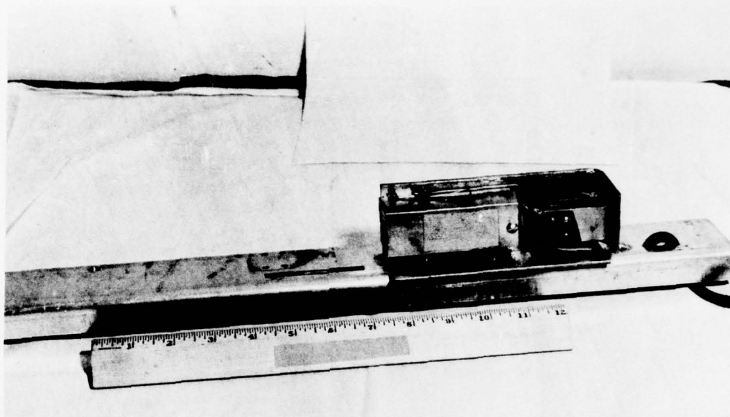
Fig. 4.11 Magnetic Trip Attached to Shutter Bar
