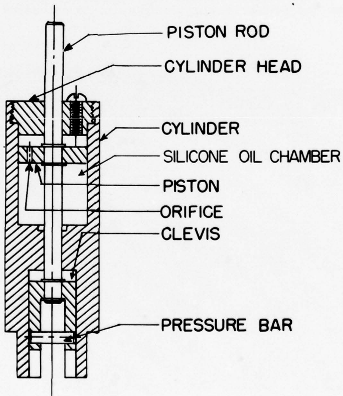
Fig. 4.9 Sectional View of Silicone Oil Timer
