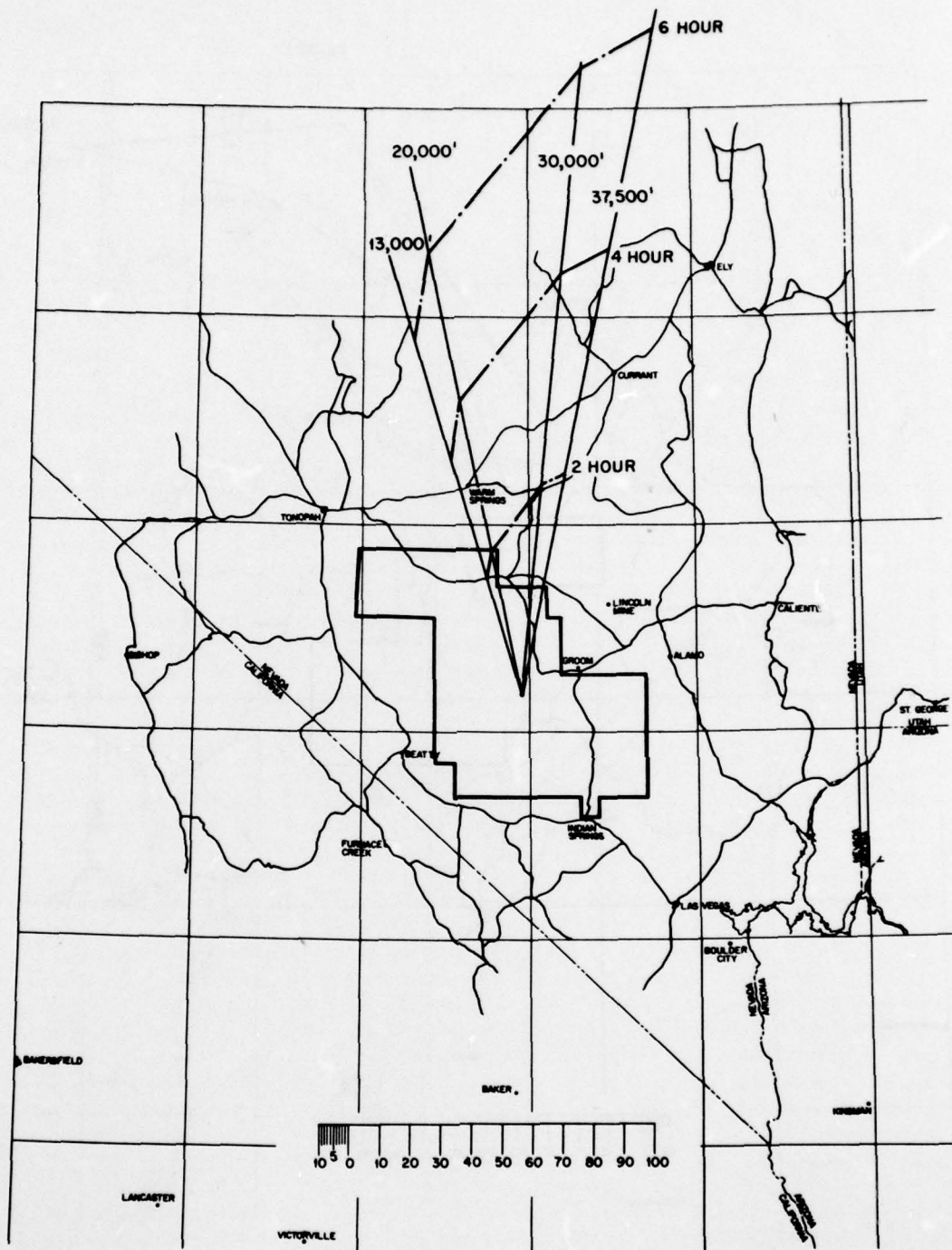
Fig. 8.1—Fall-out forecast for Tumbler-Snapper 7, prepared from 0300 winds, D-day.
