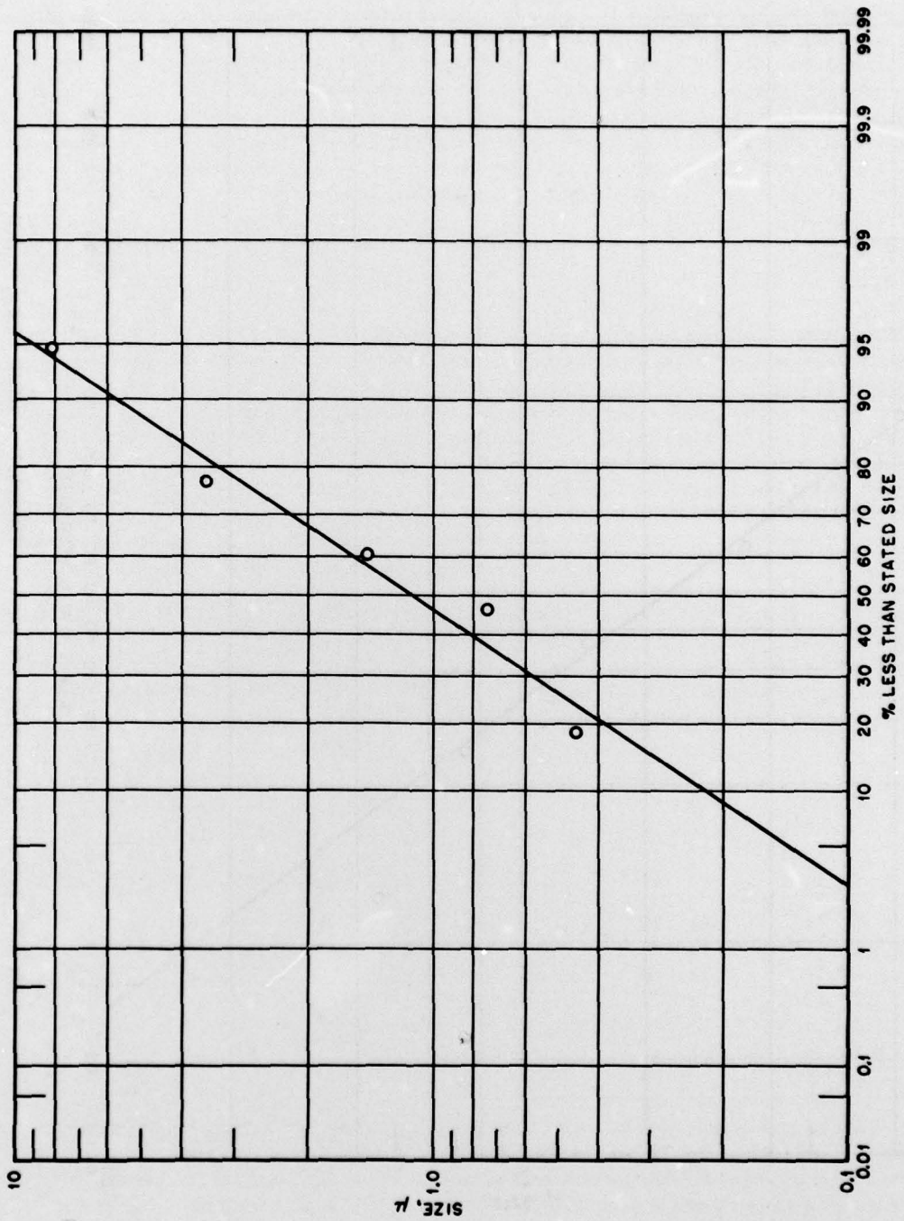
Fig. 9.4—Tumbler-Snapper 6, cascade impactor, Alamo, Nev. (MMD = 1.1 \mu , \sigma = 3.8)
