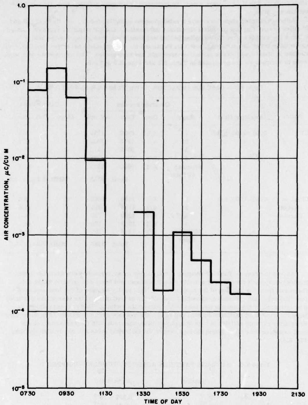
Fig. 8.4—Air concentration vs time, Tumbler-Snapper 7, 20 miles west of Currant, Nev.
