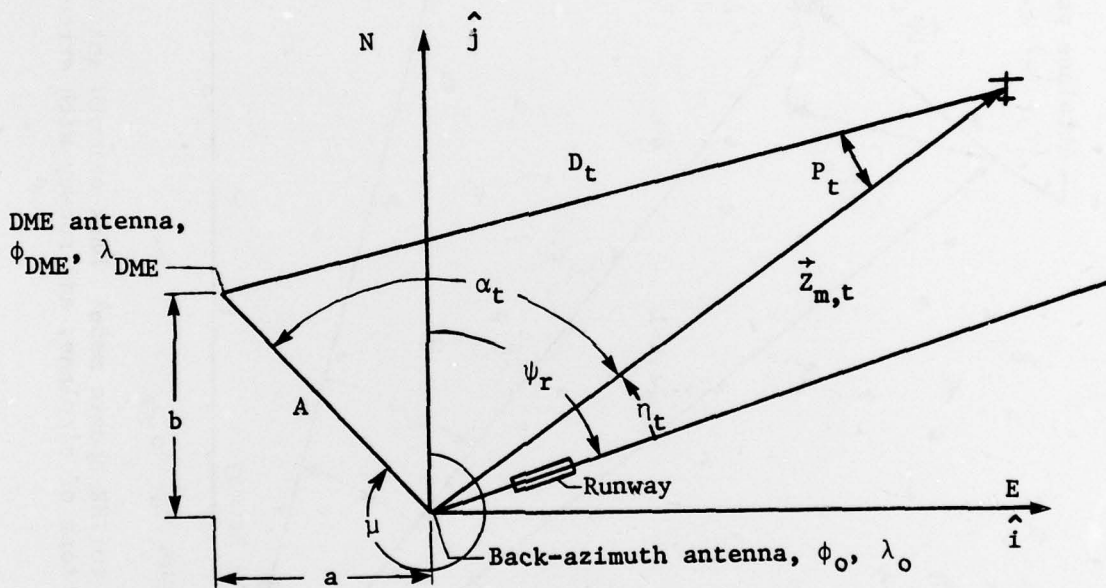
Figure 5.- Vector \vec{z}_{m,t} triangle components; IBD update mode.
