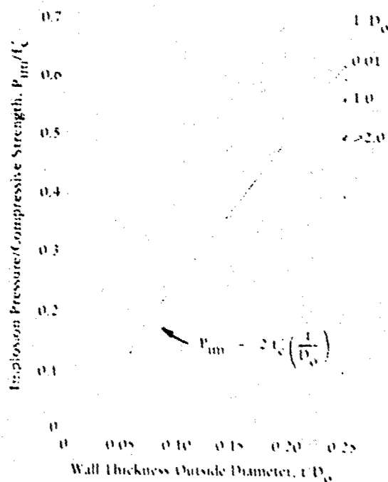
Figure 2. Relationship of Equation 3 for thick walled cylinders
