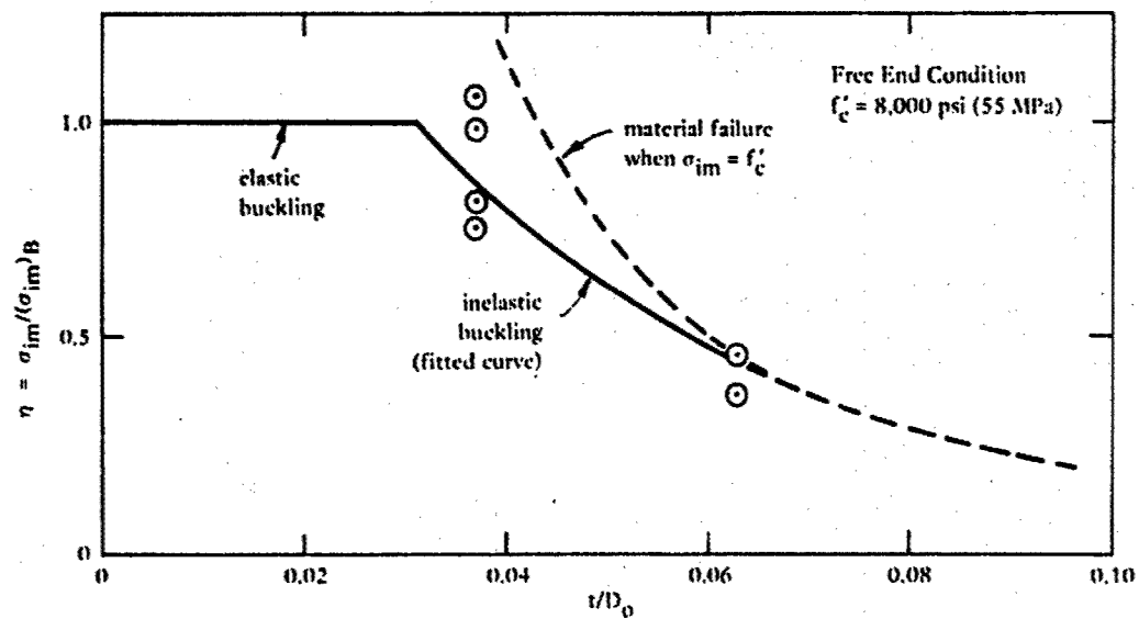
Figure 6. Implosion of long cylinder specimens with D_0 = 54 in. (1372 mm).
