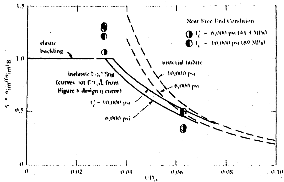
Figure 7. Implosion of long cylinder specimens with D_o = 16 in. (406 mm) (after Ref 4).
