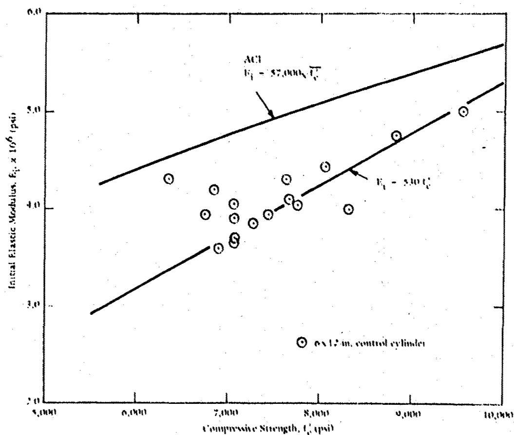
Figure 4 Relationship between E_i and f'_c .
