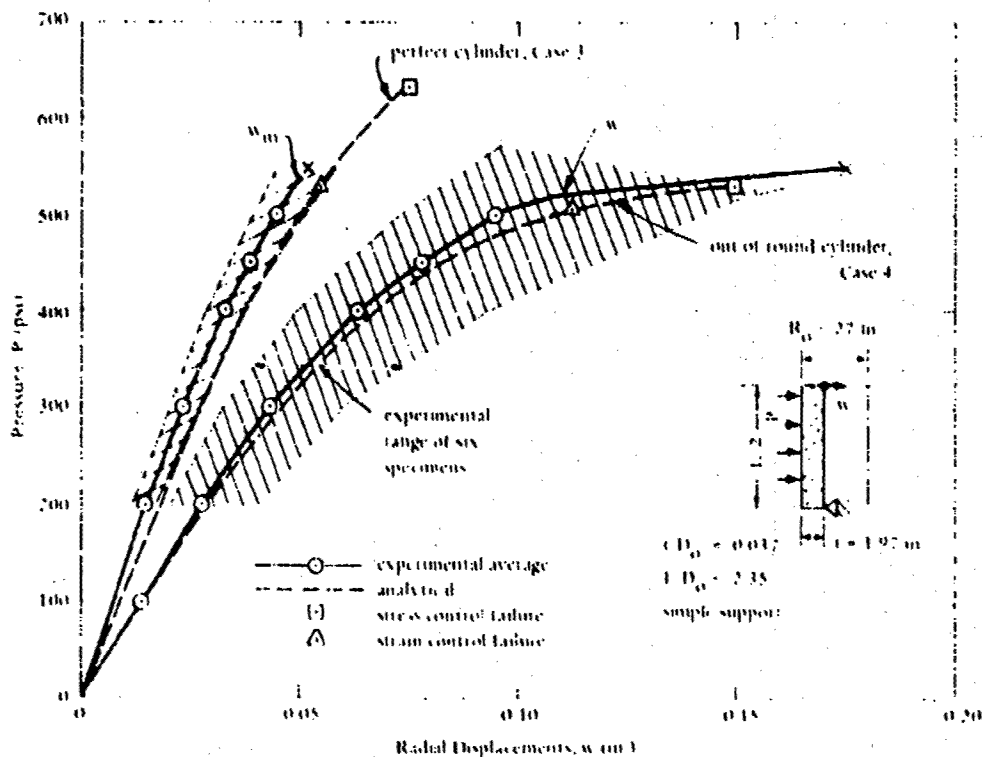
Figure B.22 Radial displacement behavior at midlength of Group 3 cylinders having t/D_o = 0.037 and simple support
