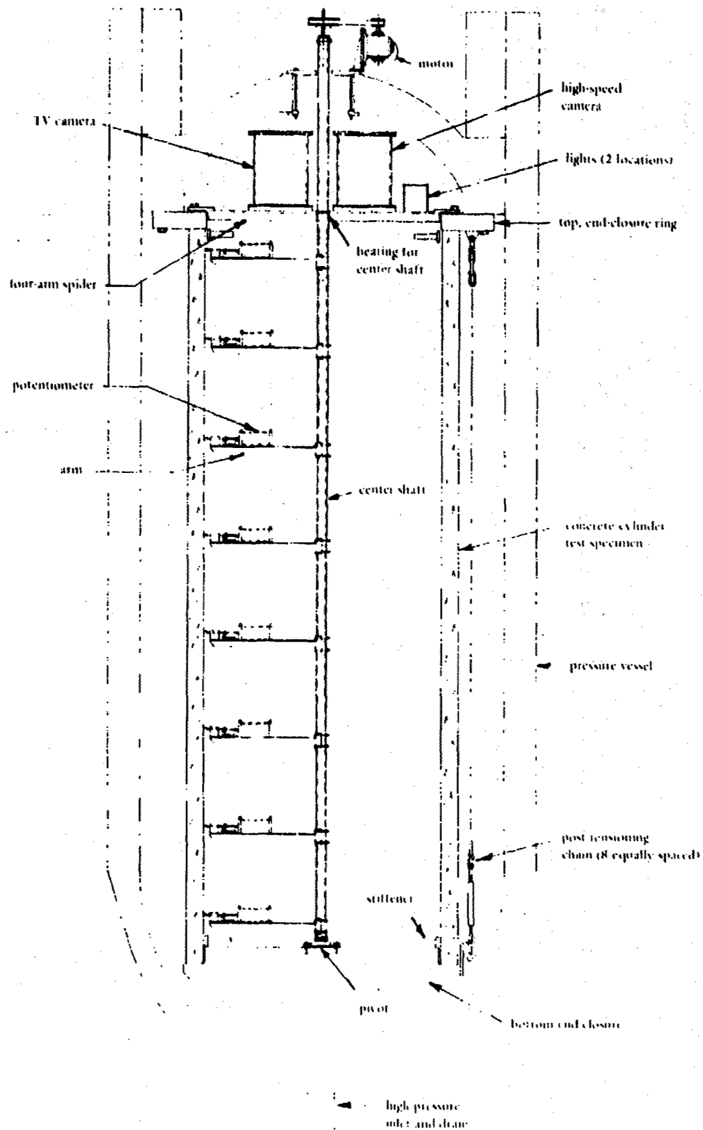
Figure B.3. Cross section of specimen, showing test setup
