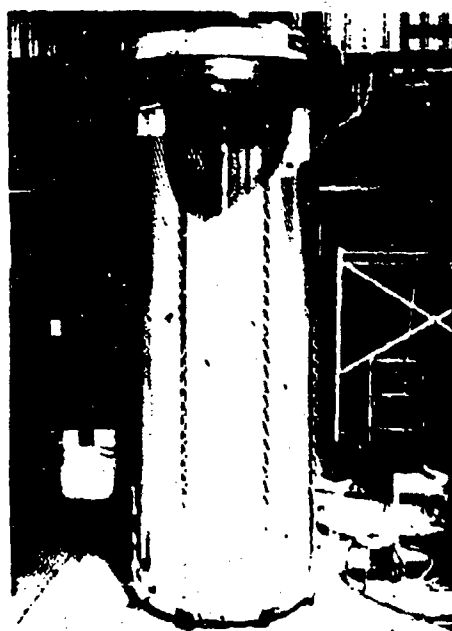
Figure B-11 Post-implosion view of specimen 2.2 at D_{50} = 0.037 (see support)
