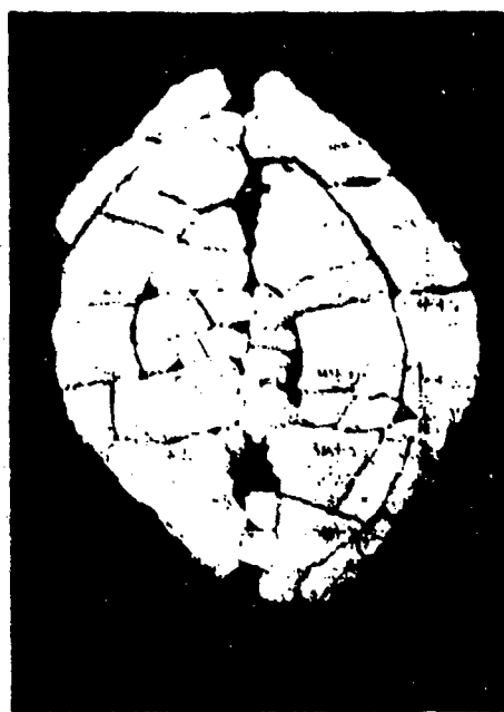
Figure B-9 Fragments of failure hole from specimen 1.1
