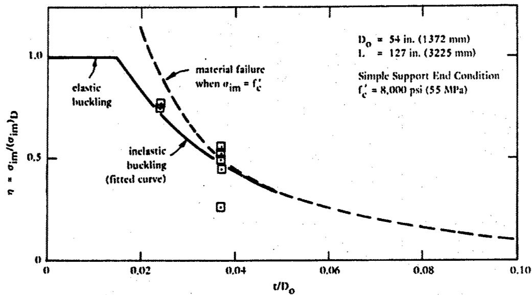
Figure 5. Implosion of moderately long cylinder specimens with D_0 = 54 in. (1372 mm).
