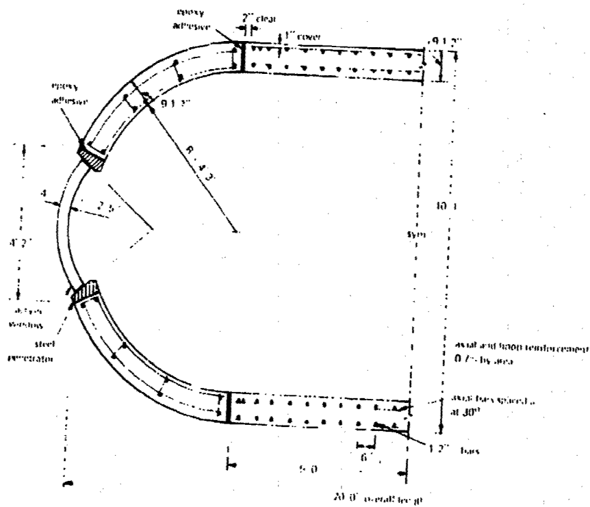
Figure A-1: SEACON structure prepared for ocean test to implosion.
