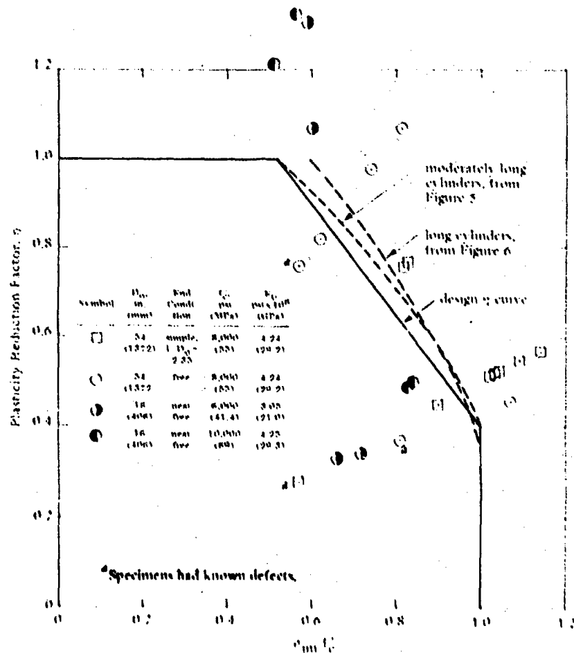
Figure 8. Plasticity reduction factor as a function of stress level in cylinder wall at implosion
