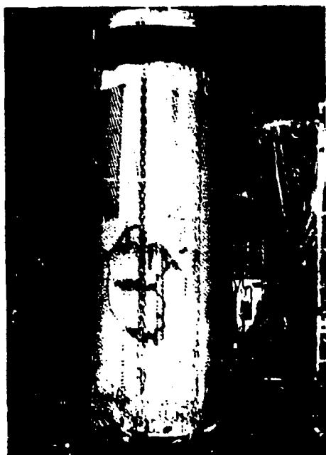
Figure B-8 Post-implosion view of specimen 1.1 at D_{50} = 0.021 (see support)
