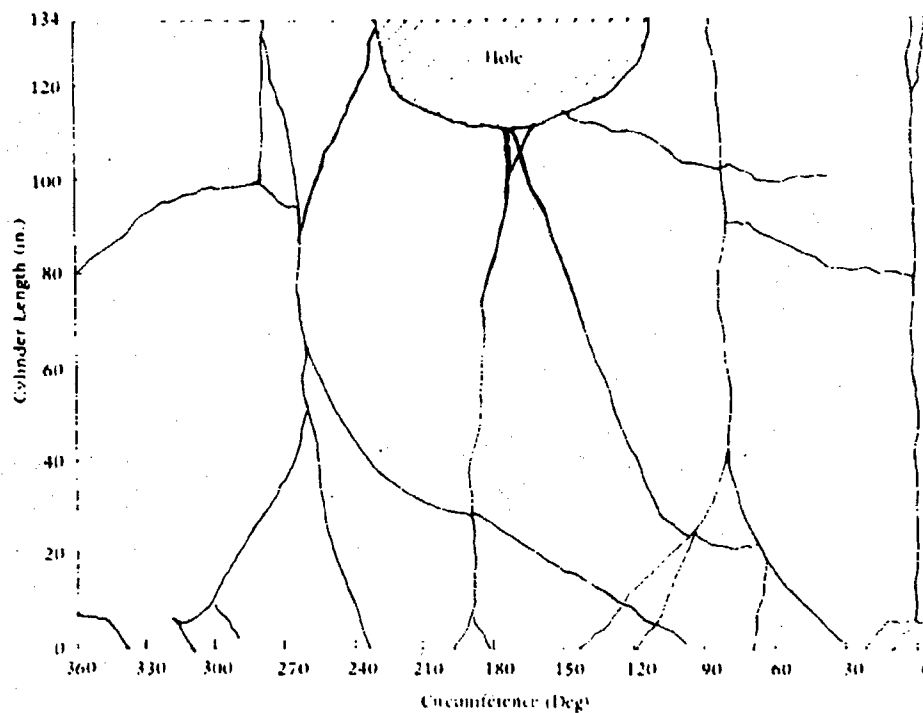
Figure B-15. Post-implosion view of specimen 5-1 ( t/D_o = 0.063 , free support)
