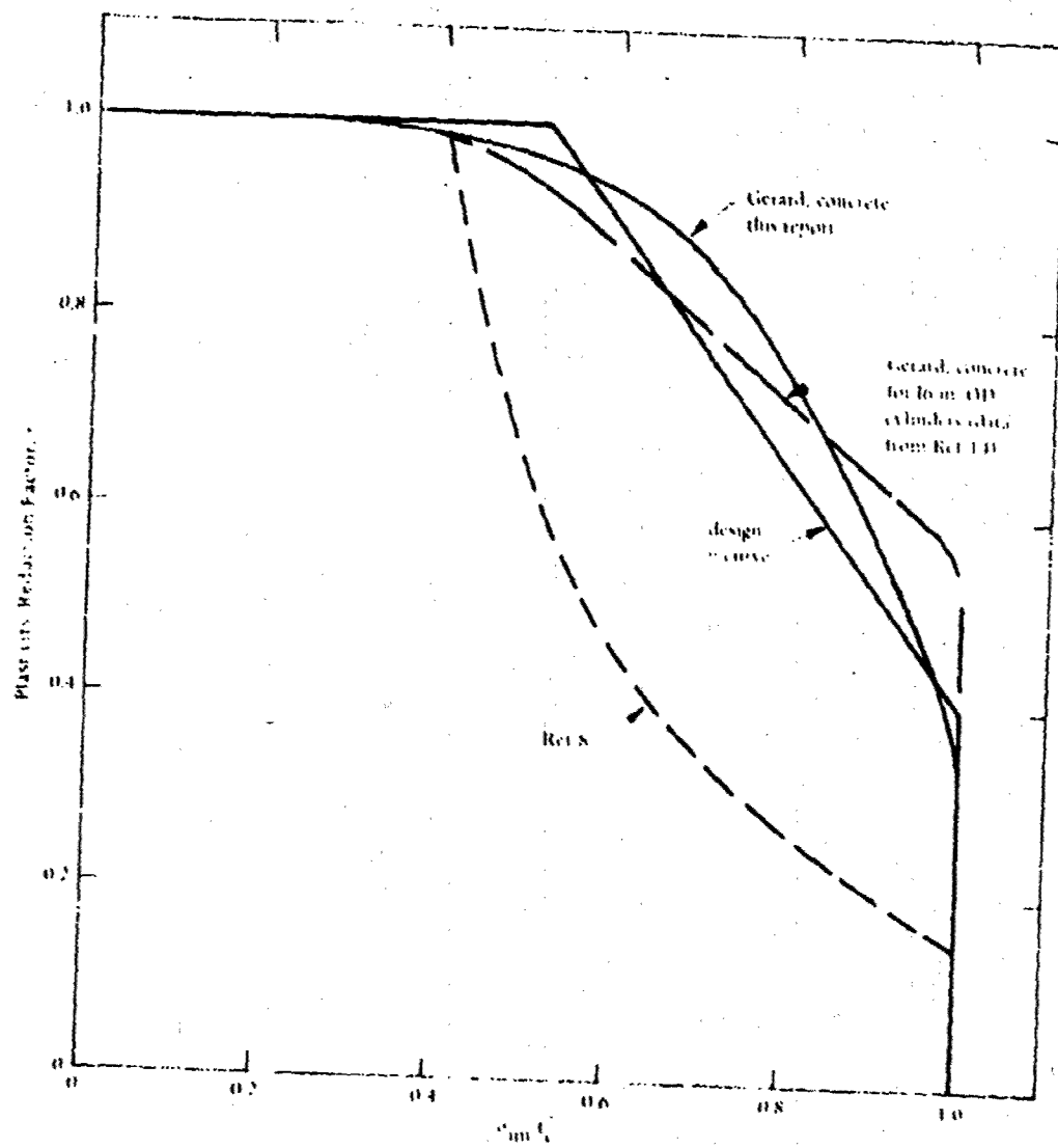
Figure 9 Comparison of various \eta versus \sigma_{fm} / f'_c relationships
