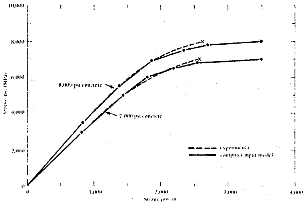
Figure B-7. Uniaxial compressive stress-strain relationship for concrete
