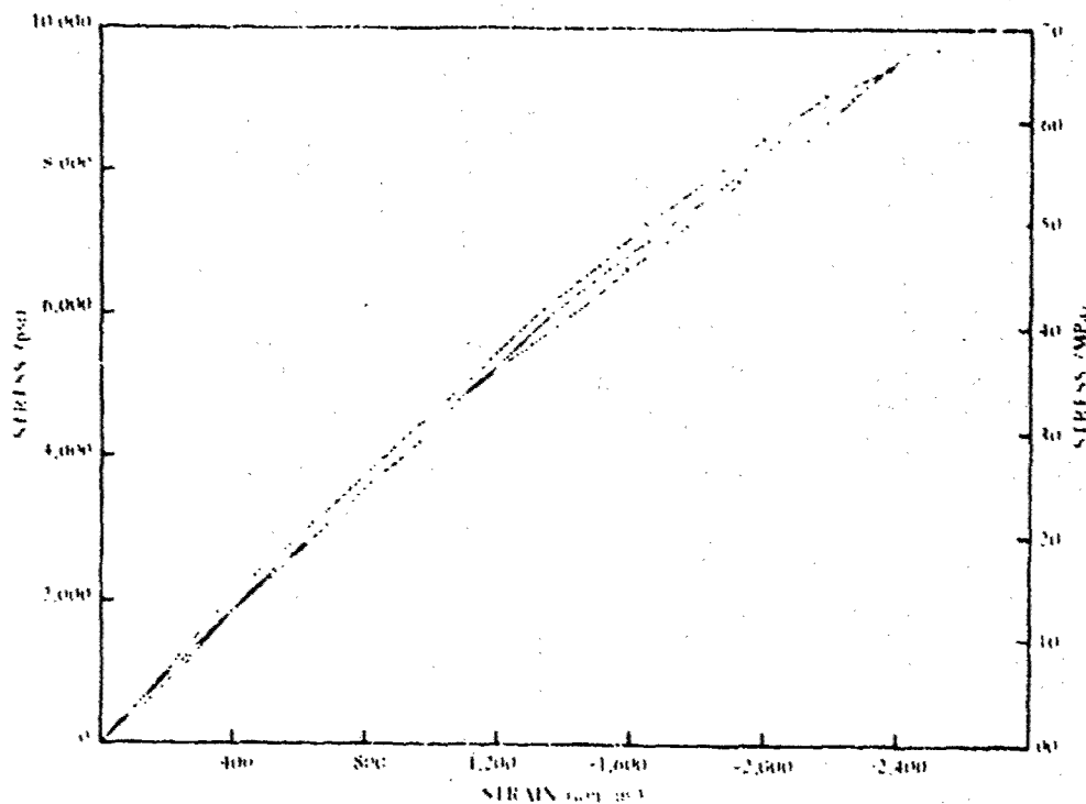
Figure A 3. Stress-strain curves from 3.25-in. diam x 6-in. long cores
