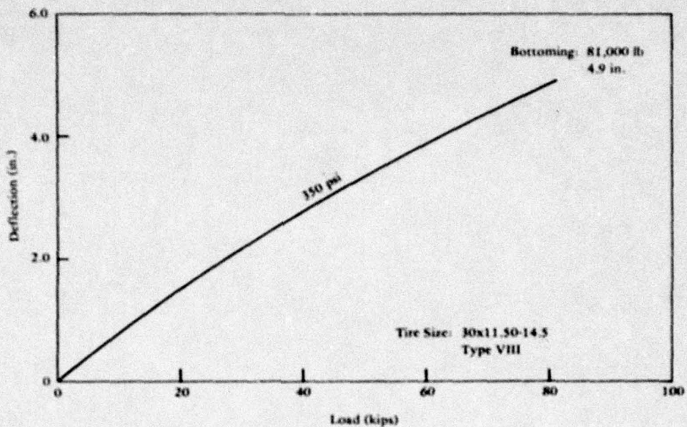
(a) Main landing gear tire load deflection diagram for F-4 (Ref 27).
