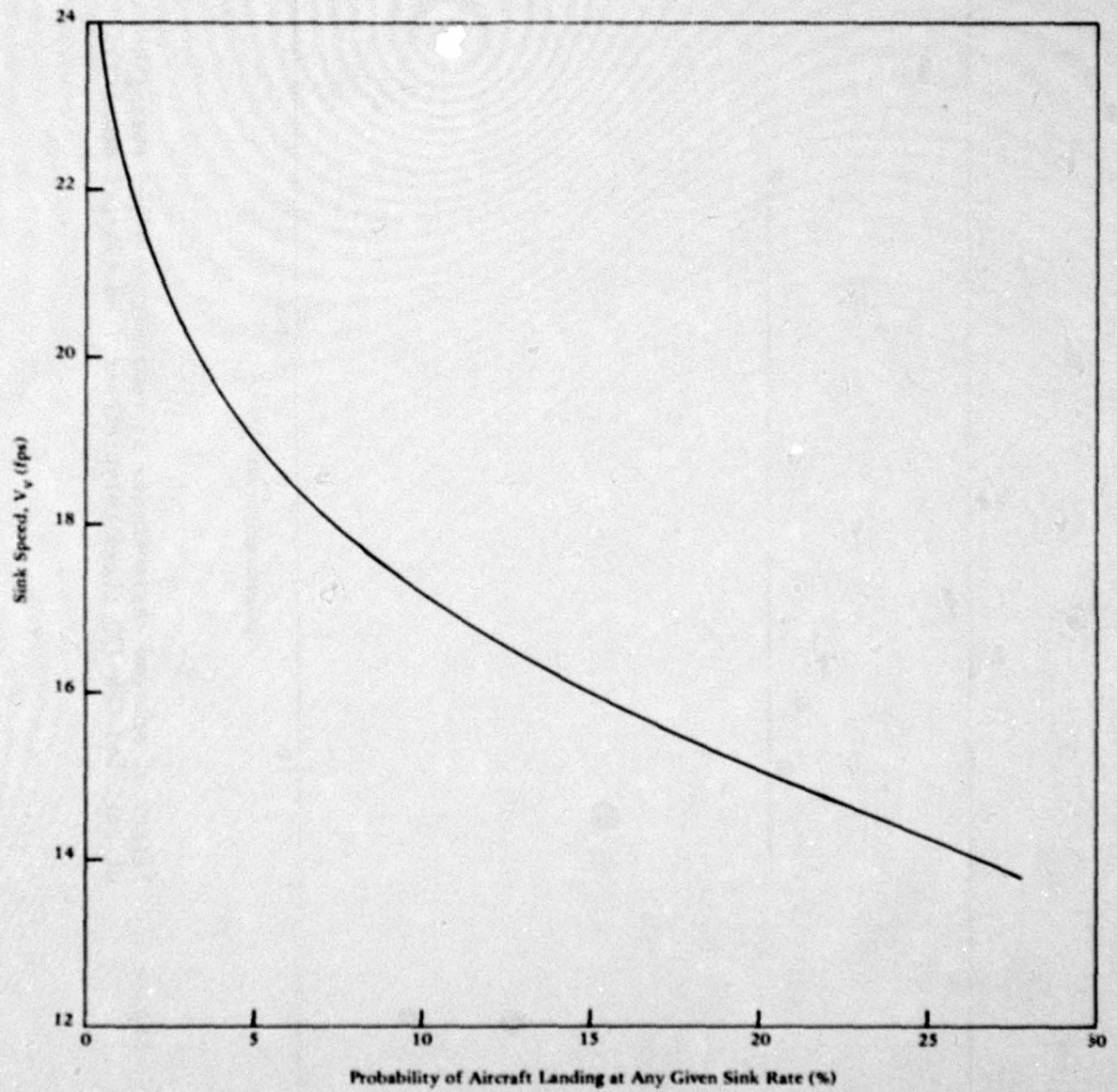
Figure 18. F-4 sink rate probability (Ref 18).
