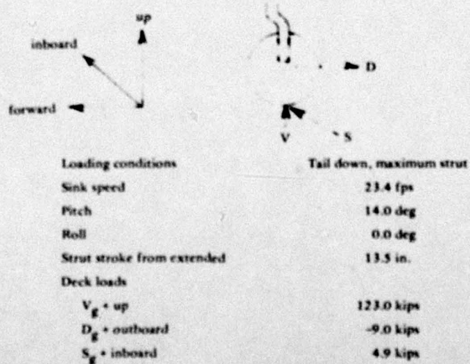
(b) F-4 main landing gear design loads, 38,000-pound landing gross weight (Ref 27).
