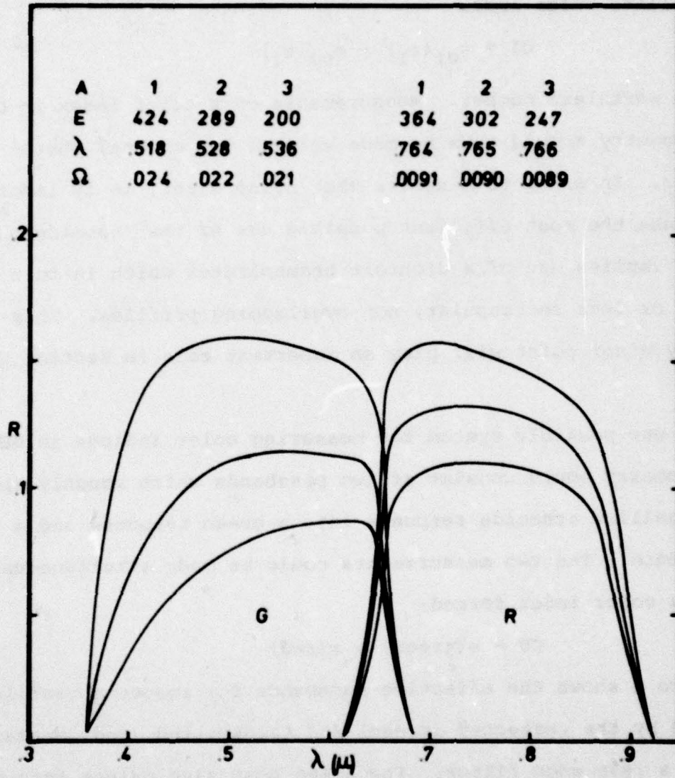
Fig. 4. The effective response profiles for two-color MBP.
