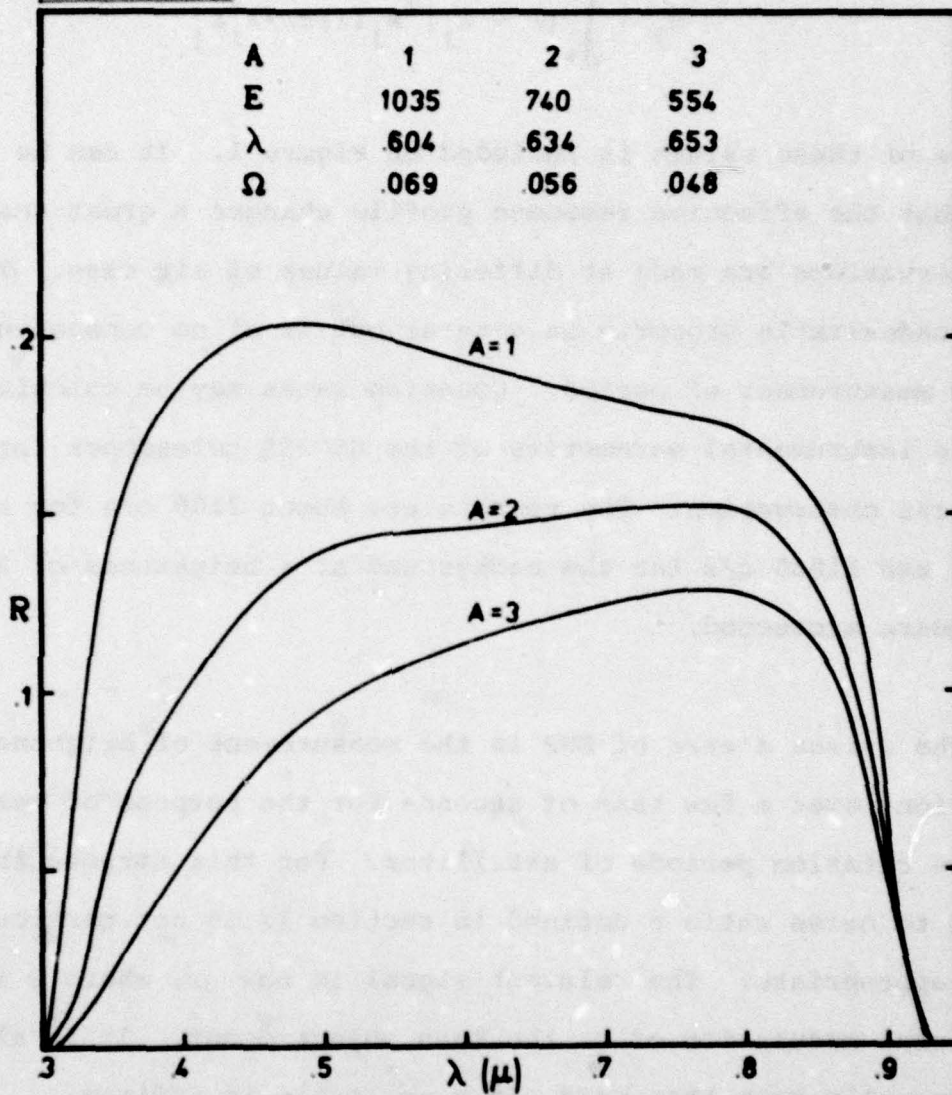
Fig. 1. The effective EWP response profiles for observations through differing values of the air mass, A. The total throughput (in equivalent Angstroms), the central wavelength (in \mu ) and the dimensionless r.m.s. width are tabulated.
