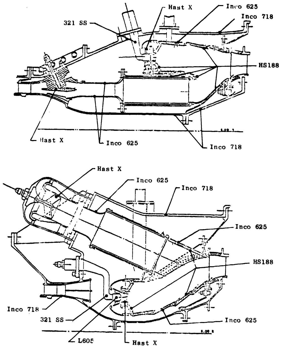
Figure 37. Catalytic Combustor Materials.
