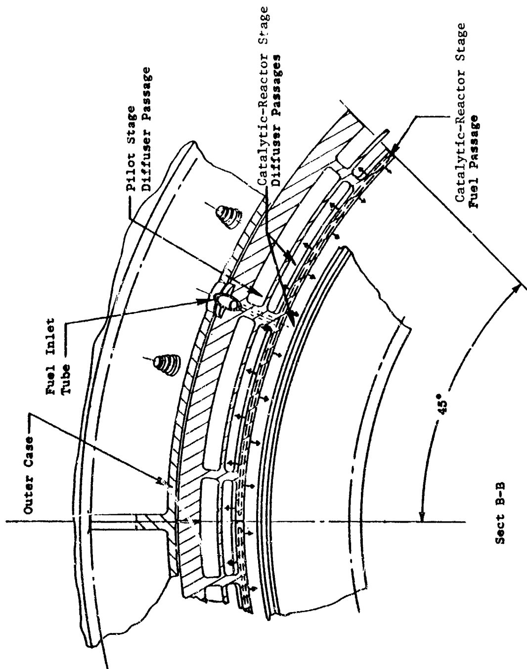
Figure 24. Basic Parallel-Staged Combustor Fuel-Injector/Diffuser.
