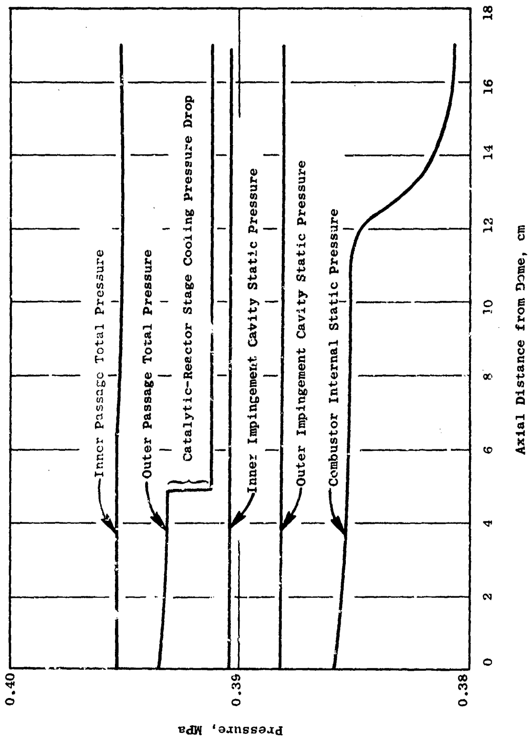
Figure 39. Combustor Pressure Distributions for the Cannular, Reverse-Flow Parallel- Staged Catalytic Combustor (Idle Power).
