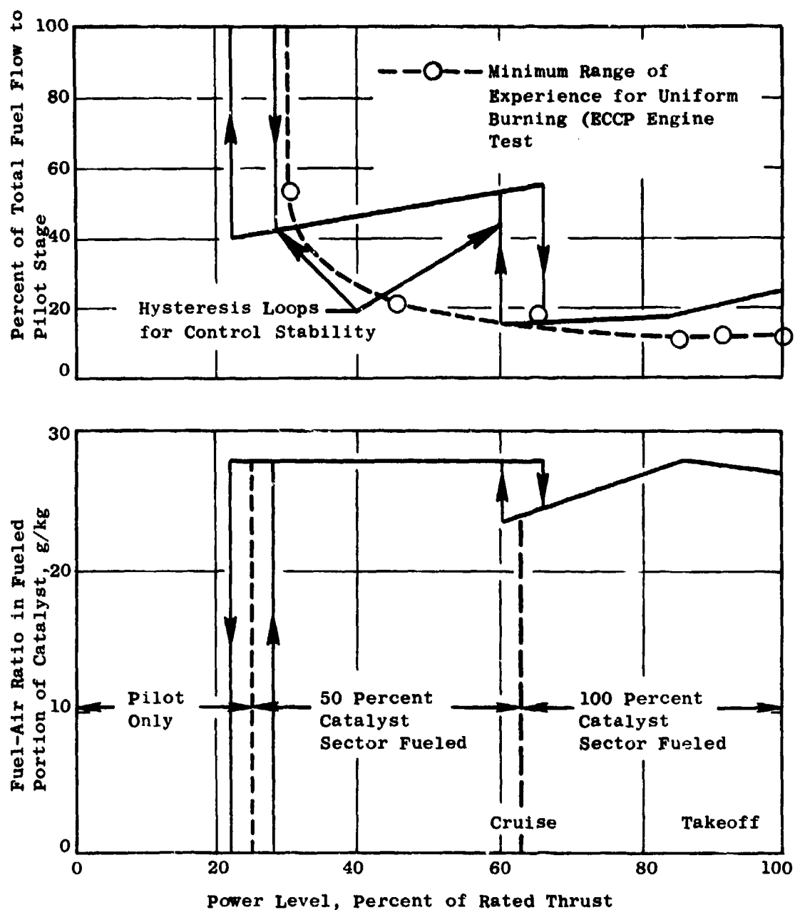
Figure 35. Cannular Reverse-Flow Combustor (Concept 4) Fuel-Flow Schedules.
