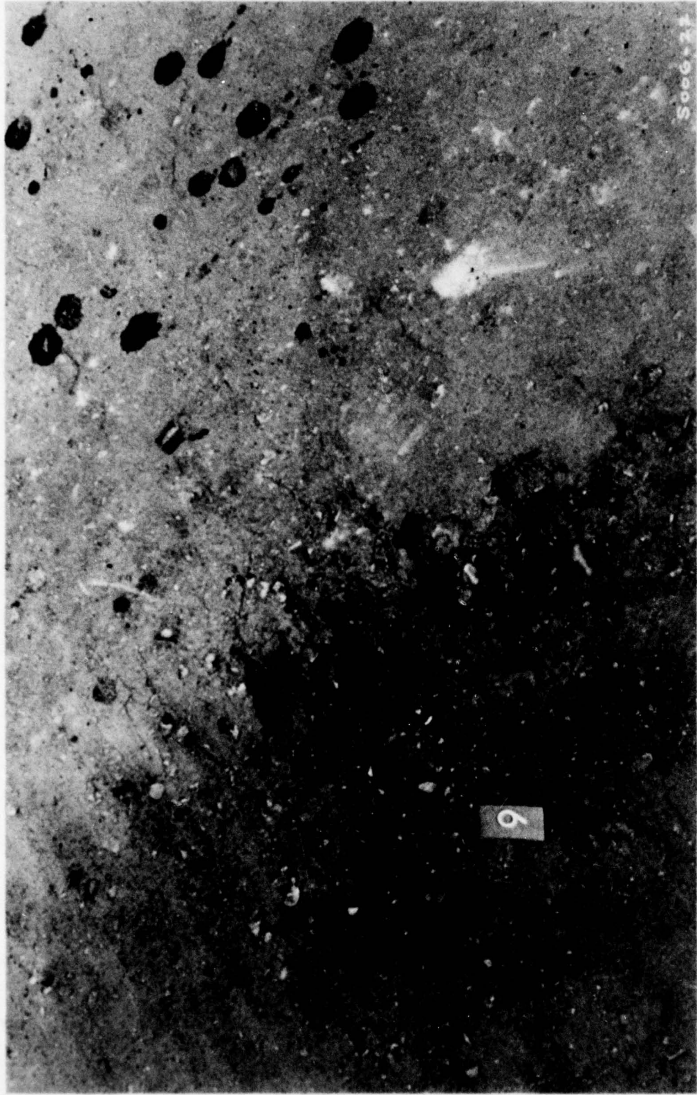
Photo 41. Close-up of outside wheel path in item 9 indicating tire impressions after 1450 operations
