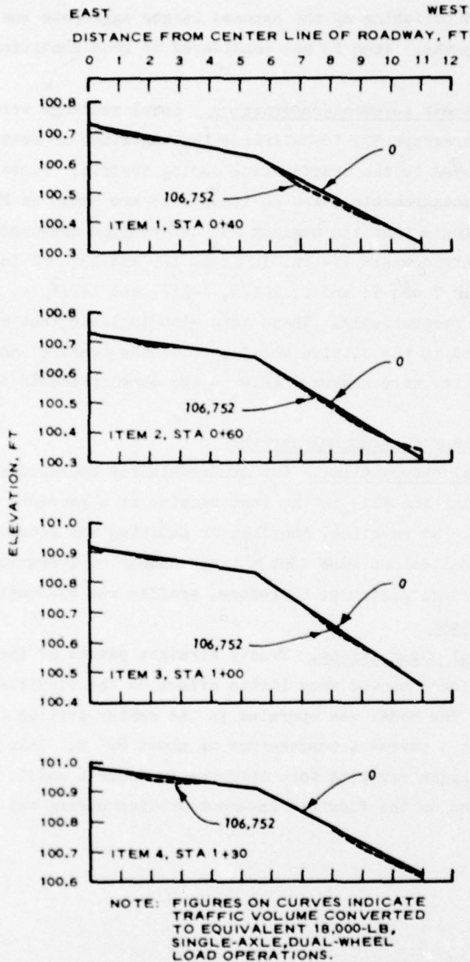
Figure 16. Typical cross sections of items 1-4, lane 2
