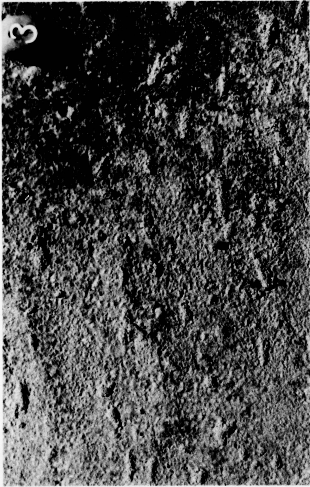
Photo 14. Surface texture of item 4 (first concrete placement lane) after compaction
