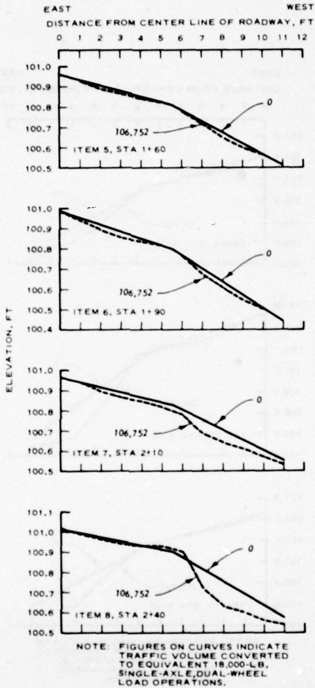
Figure 17. Typical cross sections of items 5-8, lane 2
