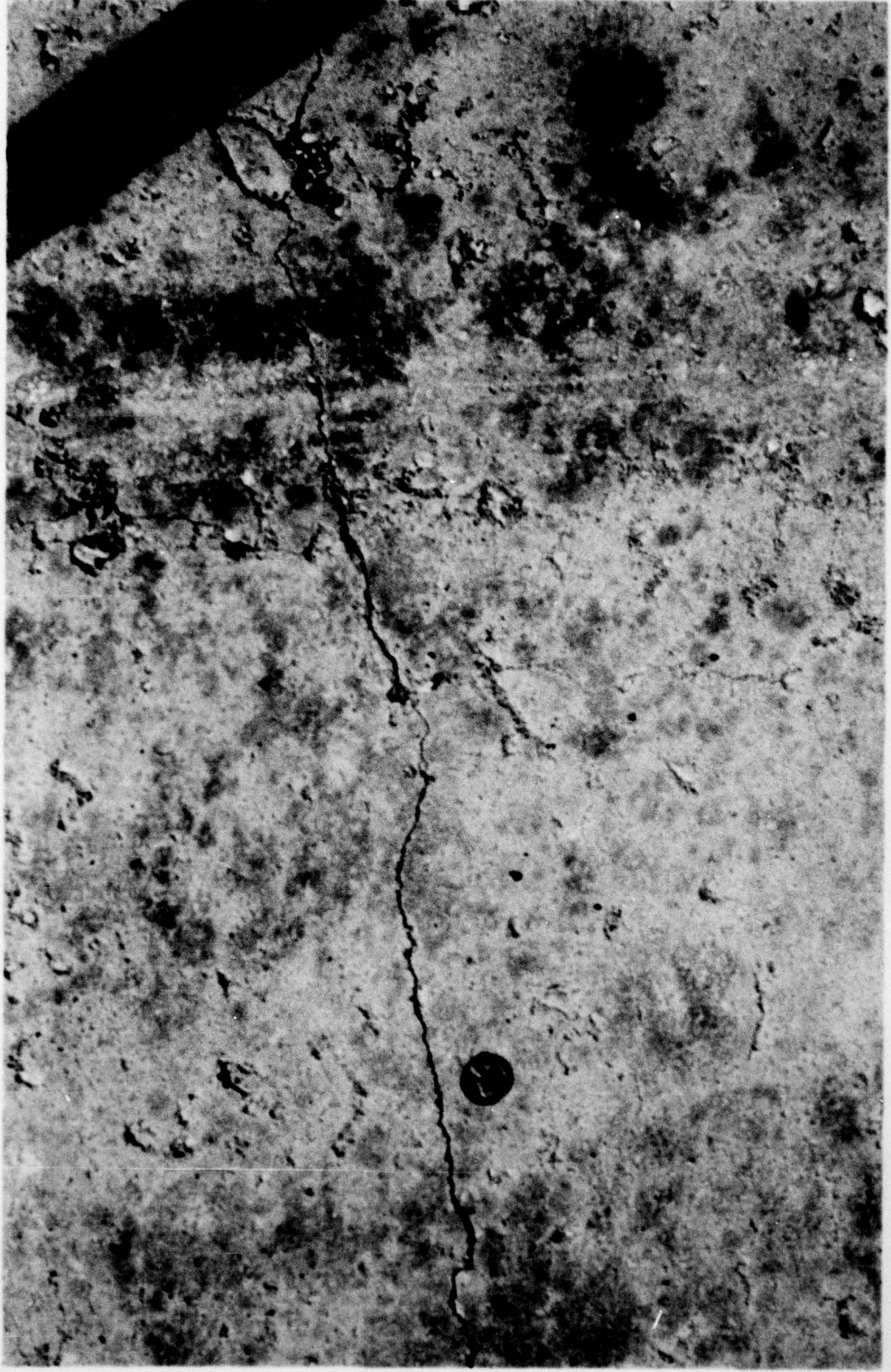
Photo 79. Contraction crack in item 6 prior to traffic
