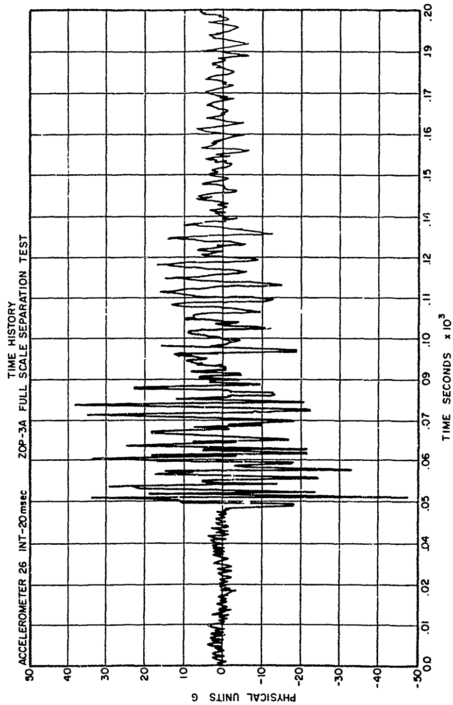
ACCELERATION HISTORY AT INTERMEDIATE LOCATION BETWEEN MISSILE JOINT
