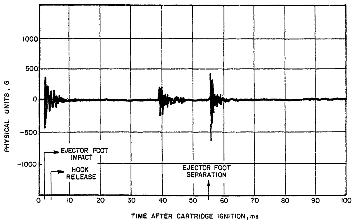
ACCELERATION HISTORY AT EJECTOR FOOT LOCATION DURING MISSILE EJECTION TEST (AERO-7A-1 RACK WITH HIGH-FORCE CARTRIDGES).
