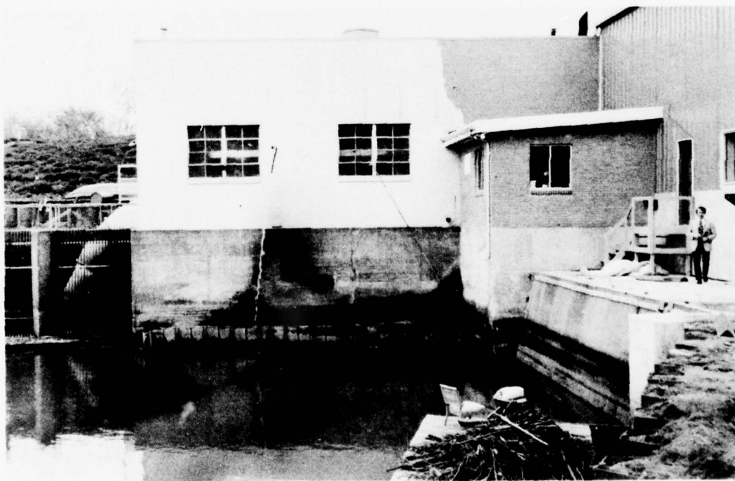
Figure 14. Entrance to sump, irregular entrance conditions, pump on left operating
