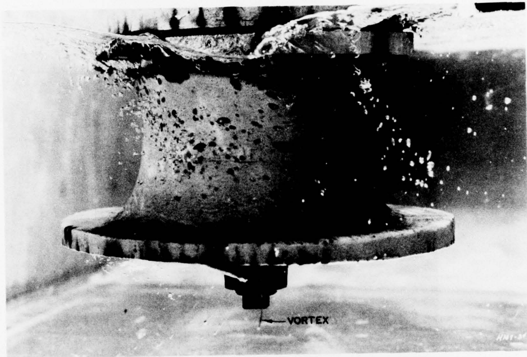
Figure 31. Submerged floor vortex, 3000-gpm discharge, 0-ft submergence
