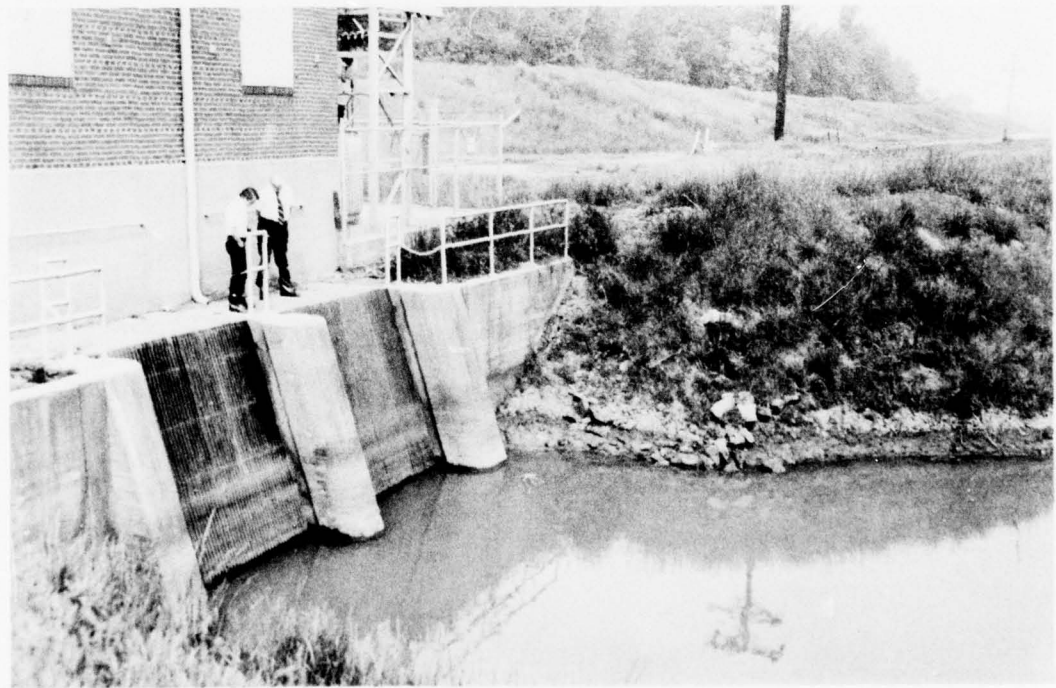
Figure 10. Entrance to sump, 90-deg wing walls, rounded pier noses, pumps not operating
