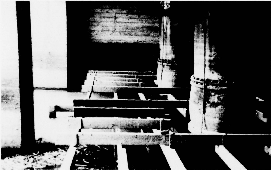
Figure 25. Floating wooden grid to minimize vortex development
