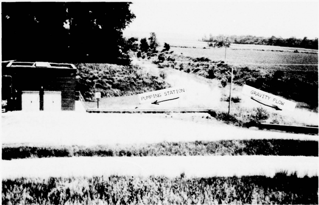
Figure 8. Pumping station and approach channel offset from gravity flow section
