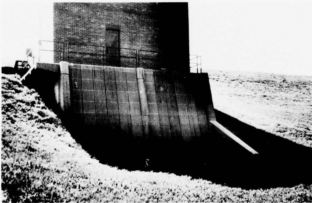
Figure 16. Entrance to sump, irregular entrance conditions, pumps not operating
