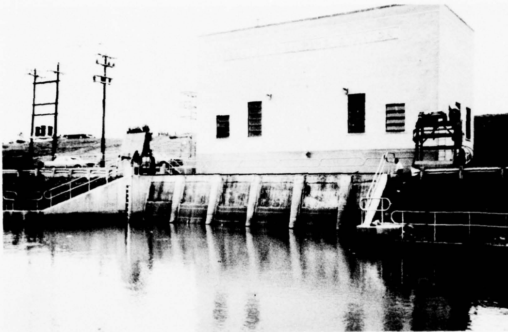
Figure 13. Entrance to sump, flared wing walls, rounded pier noses, three center pumps operating
