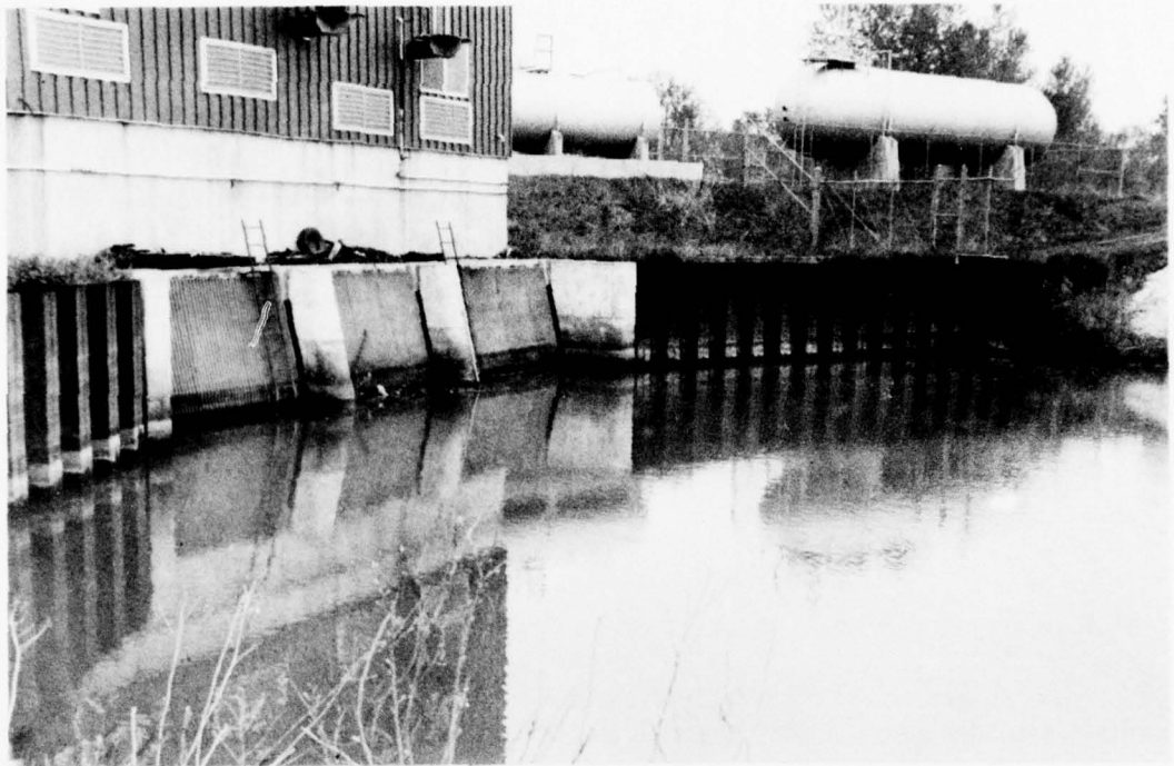
Figure 9. Entrance to sump, 45-deg wing walls, rounded pier noses, three pumps operating
