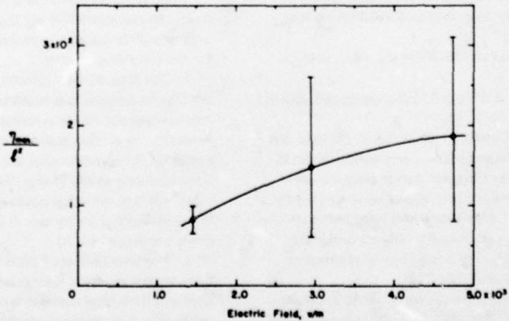
Figure 6. \eta_{\max}/R^2 vs field strength. Open circle is mean of \eta_{\max}/R^2 at the field strength and vertical bars indicate the range of measured values.
