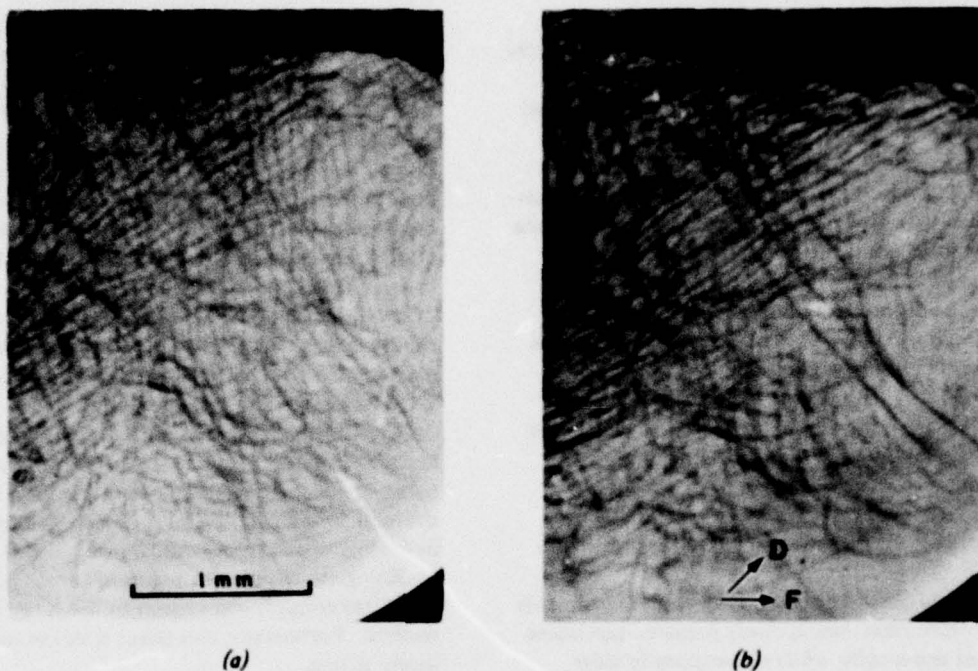
Figure 8. Comparison of dislocation image without (a) and with (b) an electric field of 32,000 V/m, 1-1/3-Hz square wave.
