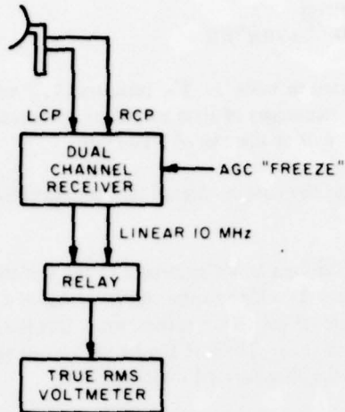
Figure 3. Antenna Figure of Merit (G/T) Configuration.
