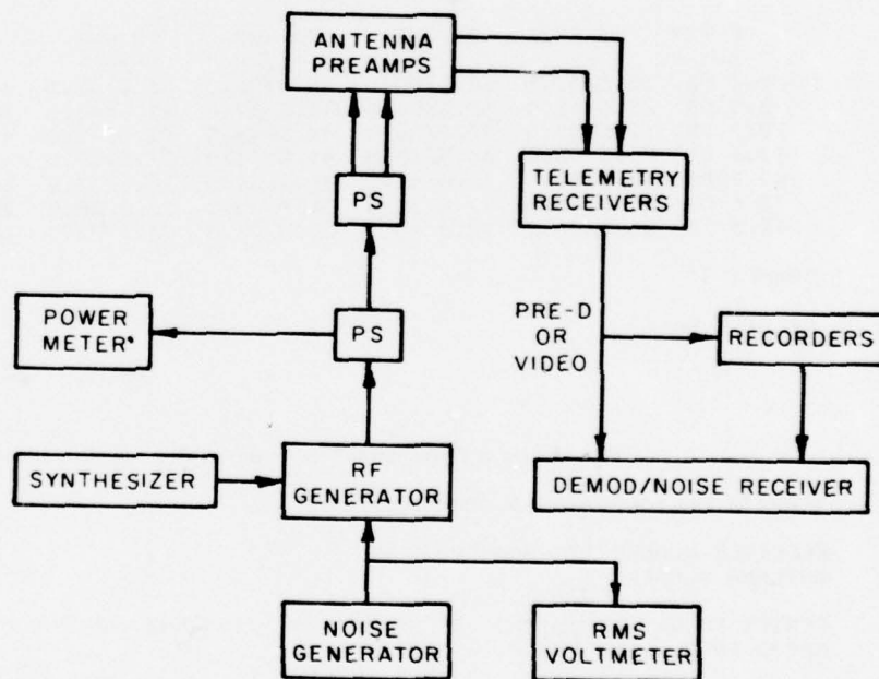
Figure 10. Noise Power Ratio (NPR) Test Configuration.
