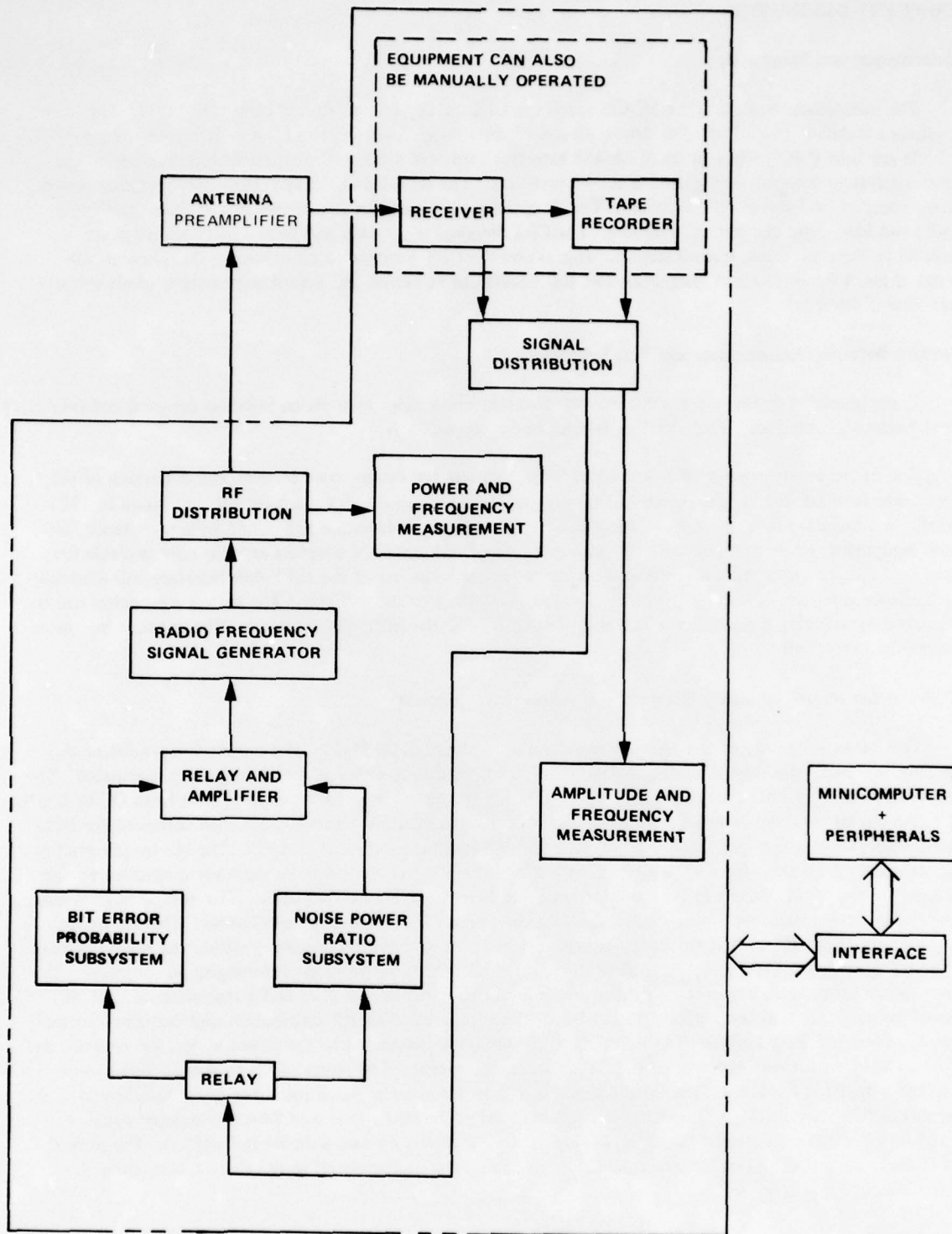
Figure 1. SCATS Block Diagram.
