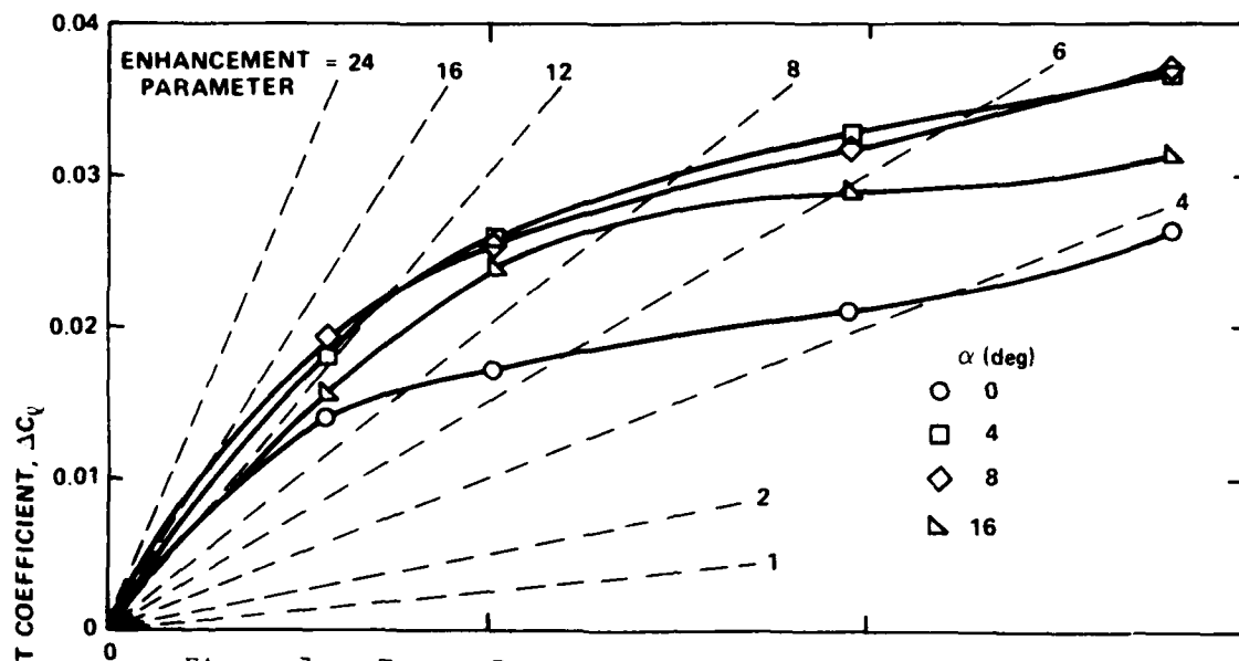
Figure 7a - Twenty-Percent CC Aileron, Simulated Short Flap
