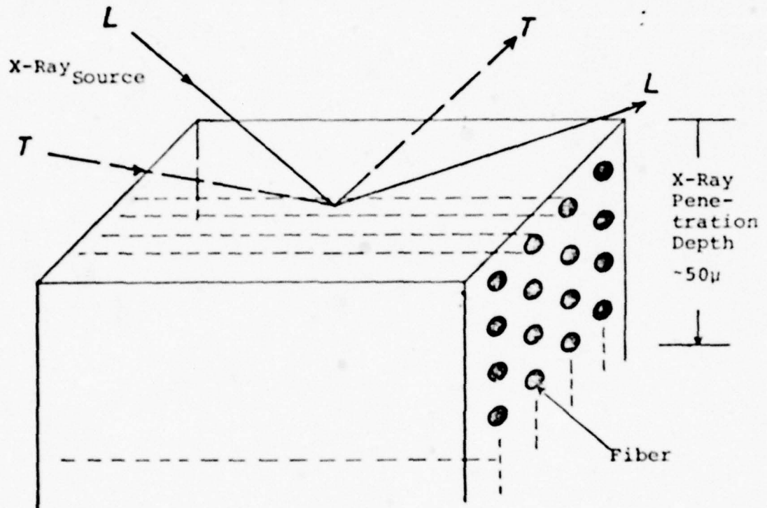
Figure 2. Measurement Geometry
