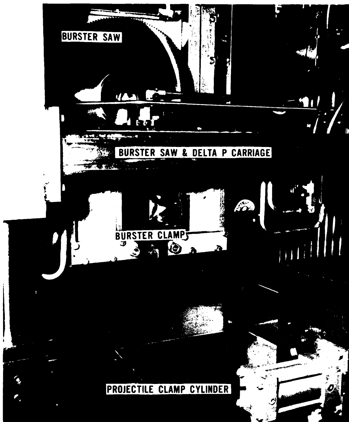
FIGURE 4-17 BURSTER SAW STATION
