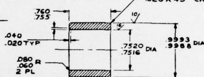
-029 INNER RACE
