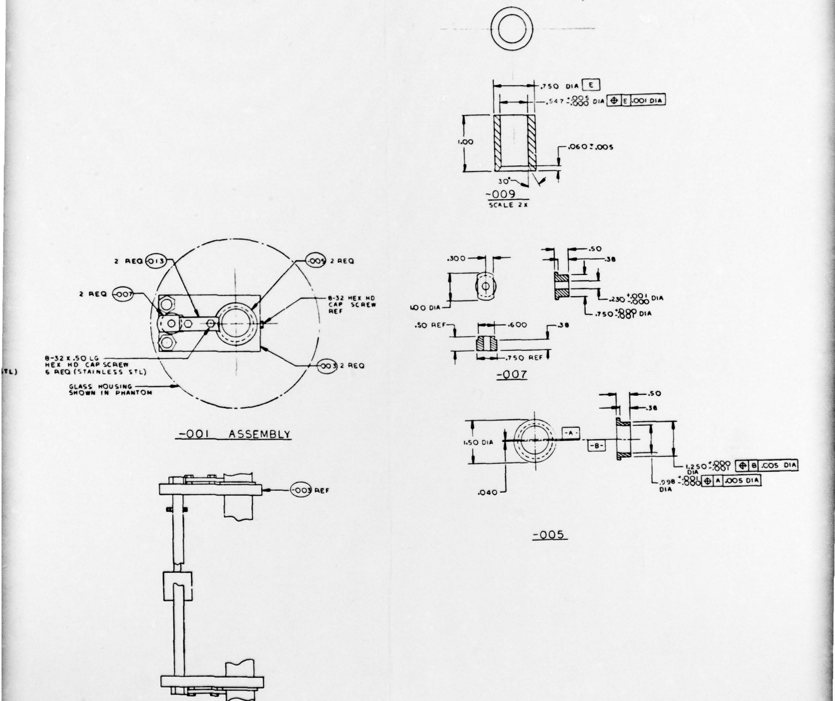
Figure 22. Small Roller Assembly
