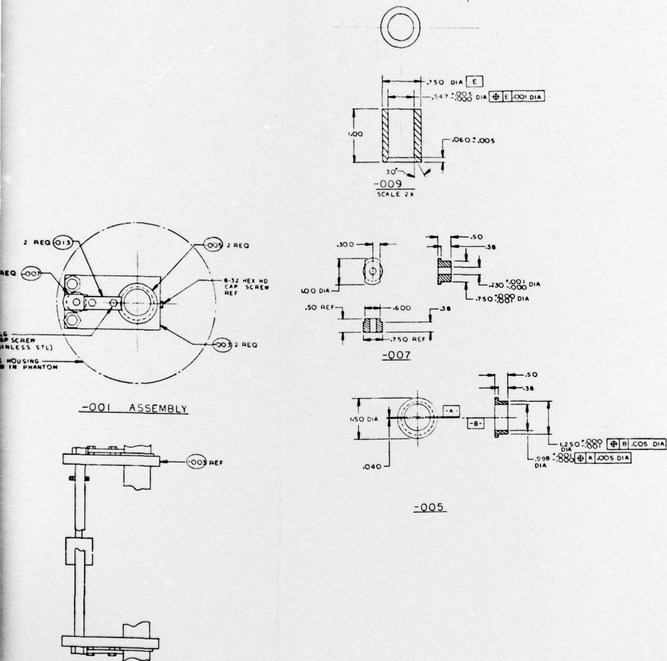
Figure 22. Small Roller Assembly
