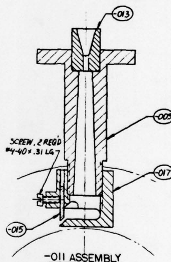
-011 ASSEMBLY
