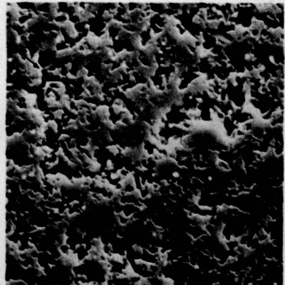
Figure 3 SEM Photomicrographs of Finished Ball Surfaces from Lot 1. Typical ball surfaces from two different balls.
