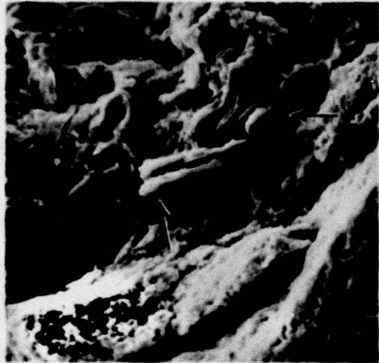
7805 1000X Unusual Particles Noted At Spall Origin
