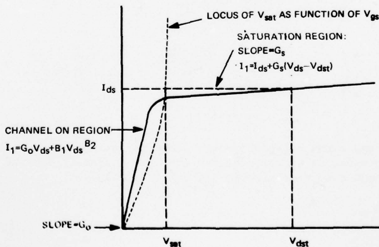
Figure 2-11. Illustration of JFET Model Parameters and Equations
