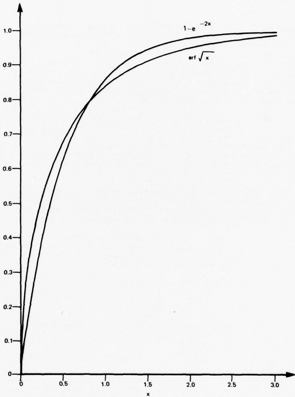
Figure 2-2. Error Function Approximation
