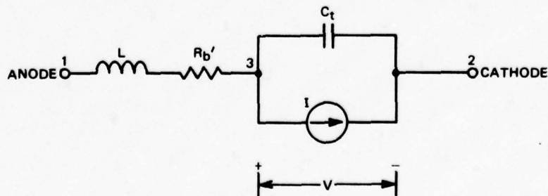
Figure 2-5. Tunnel Diode Equivalent Circuit
