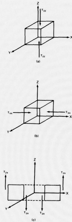
Fig. 3-2. Designation of stresses on piezoelectric ceramics
