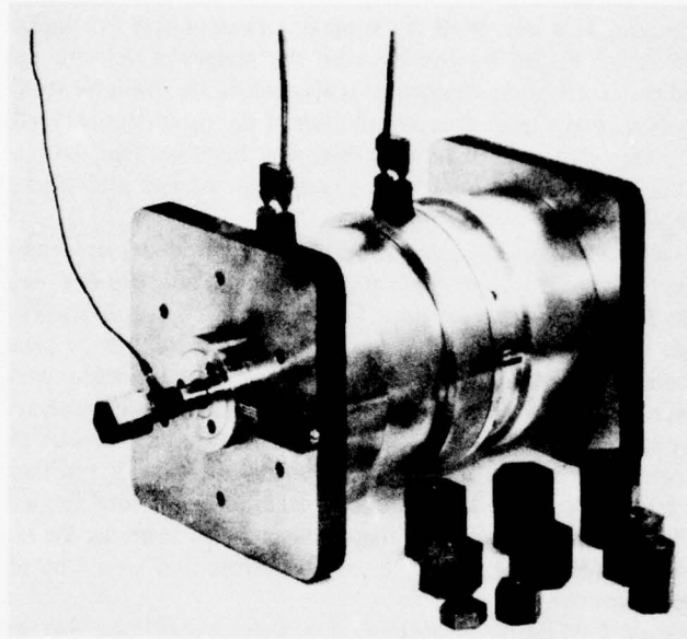
Fig. 5-9. Setup for transfer admittance measurement
