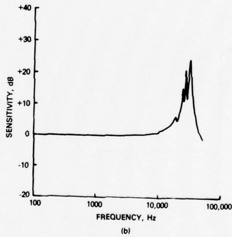
Fig. 6-8. Shock calibration of an accelerometer (a) appears normal, but (b) the resonance frequency calibration indicates internal damage [35]
