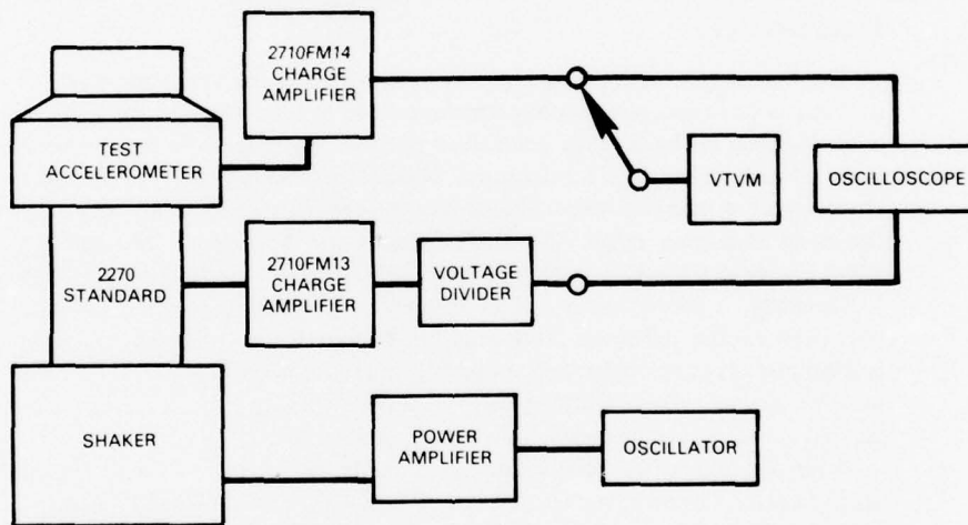
Fig. 6-1. Typical setup and block diagram for sinusoidal comparison calibration
