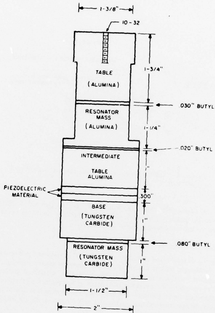
Fig. 4-4. Construction of a piezoelectric shaker [27]
