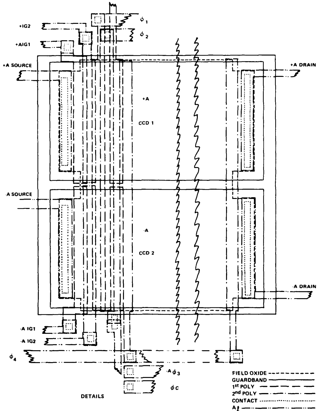
Figure 14. Differential CCD Source/Drain Details
