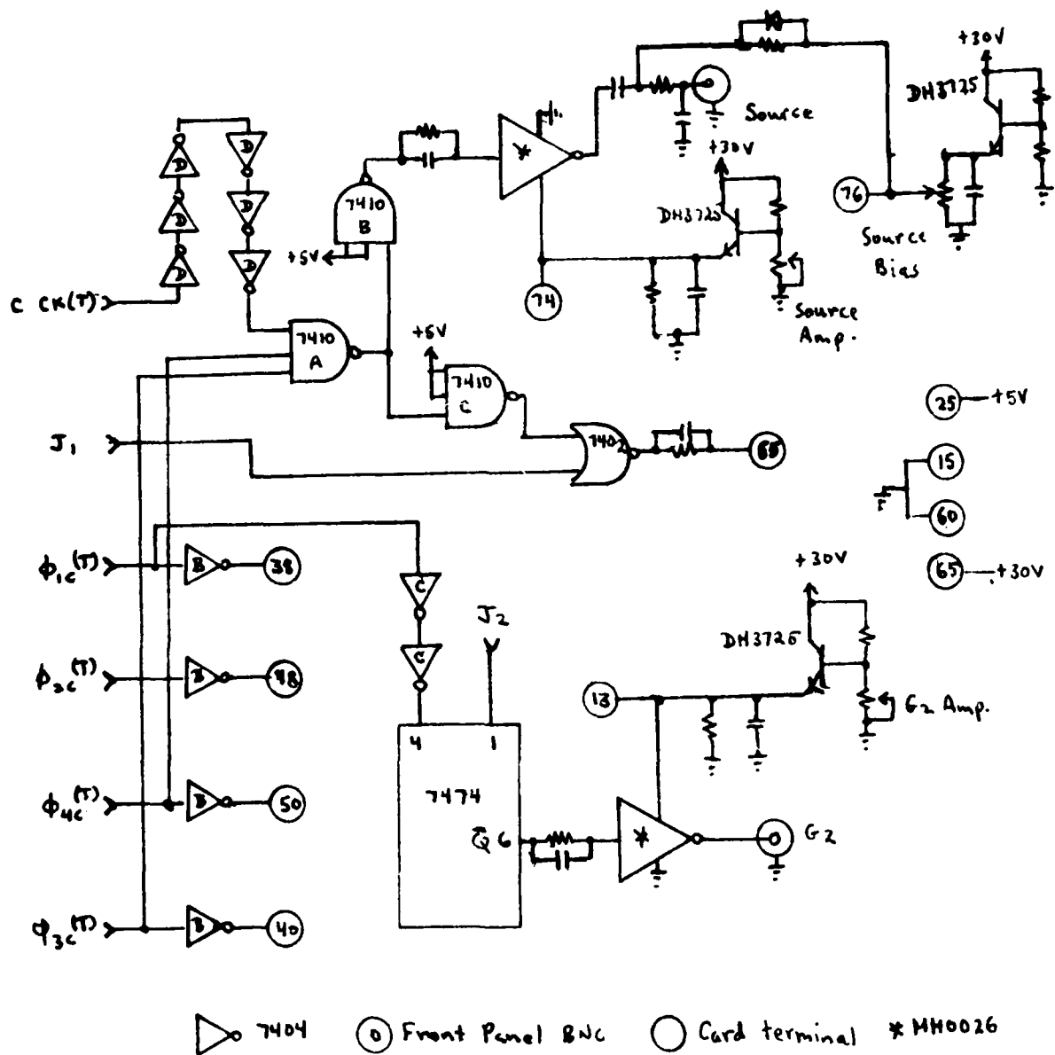
Figure 2.1(Continued) Module 2AC diagram
