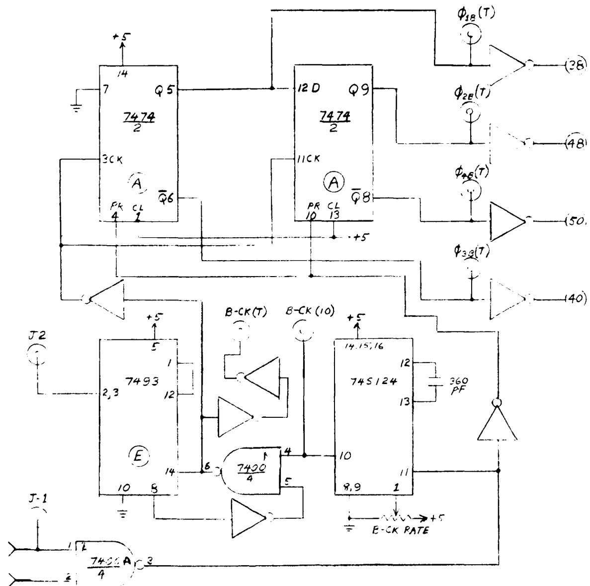
Figure 2.6 Module 2AB diagram
