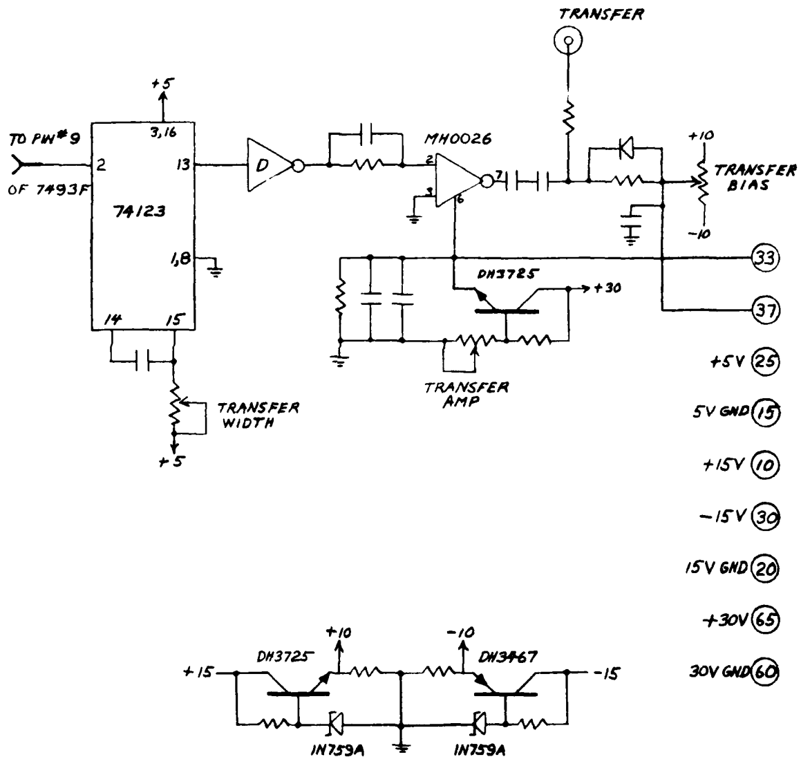
Figure 2.6 (Continued) Module 2AB diagram
