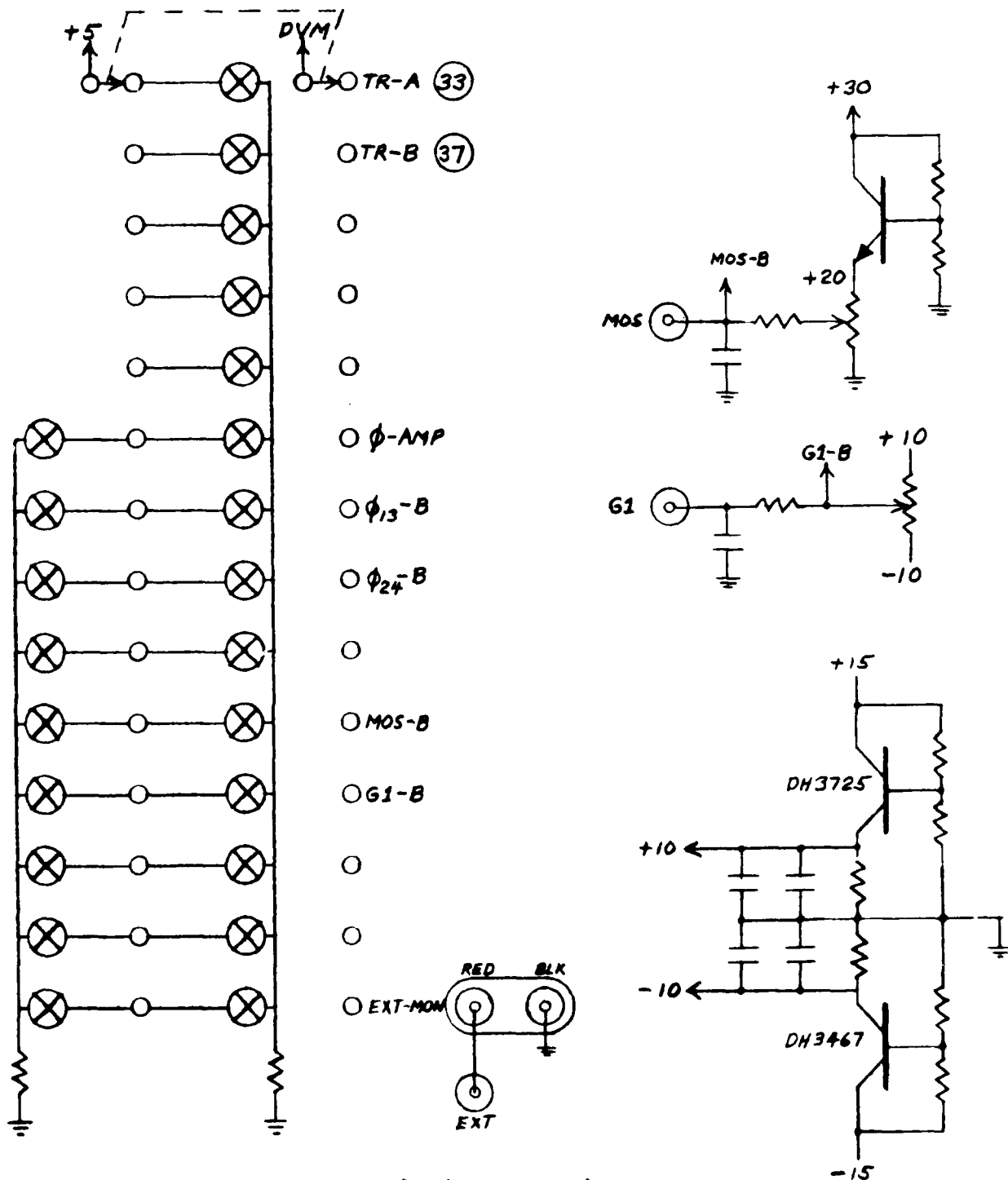
Figure 2.8 (Continued) Module 3AB diagram
