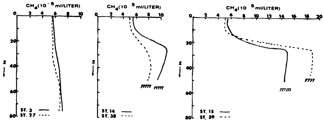
Fig. 2 — Vertical profiles of methane concentrations from the "open ocean" (stations 3 and 27), intermediate zone (stations 14 and 38), and shallow water (stations 15 and 39), with each plot showing the profiles of the two stations taken at the same coordinates
